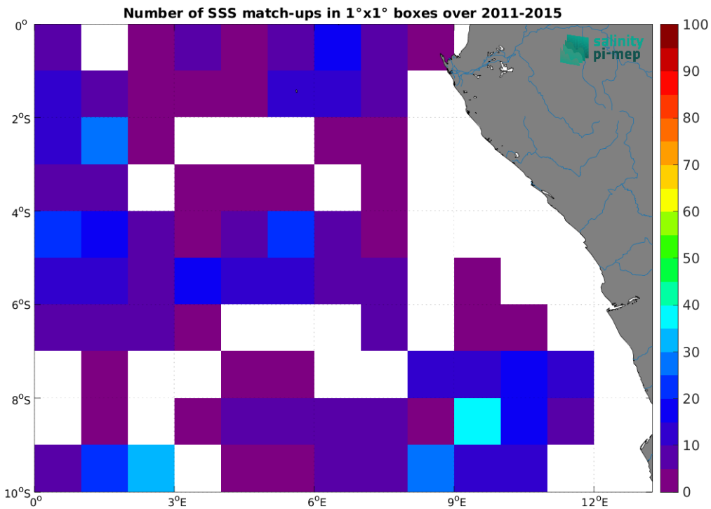
Figure 5: Number of SSS match-ups between Argo SSS and the Aquarius SSS L3 OR v5 - Monthly - Rain mask (NASA-GSFC) SSS product for the Congo river plume Pi-MEP region over 1^\circ \times 1^\circ boxes and for the full satellite product period.
