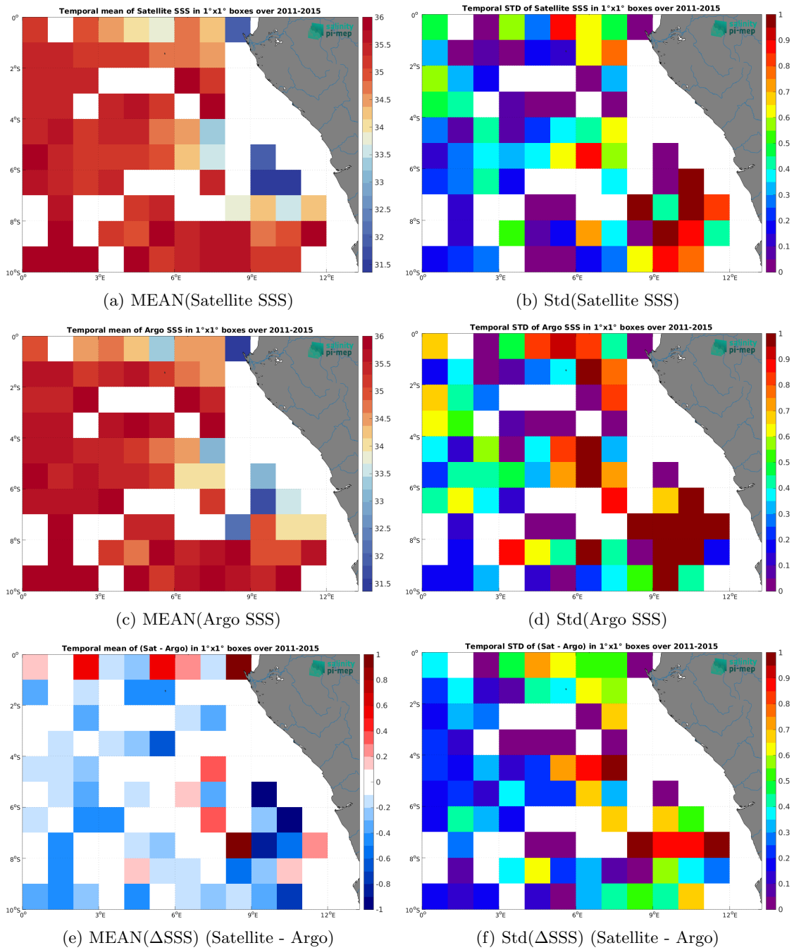
Figure 7: Temporal mean (left) and Std (right) of SSS from Aquarius SSS L3 OR v5 - Monthly - Rain mask (NASA-GSFC) (top), Argo (middle), and of \Delta SSS (Satellite - Argo). Only match-up pairs are used to generate these maps.
