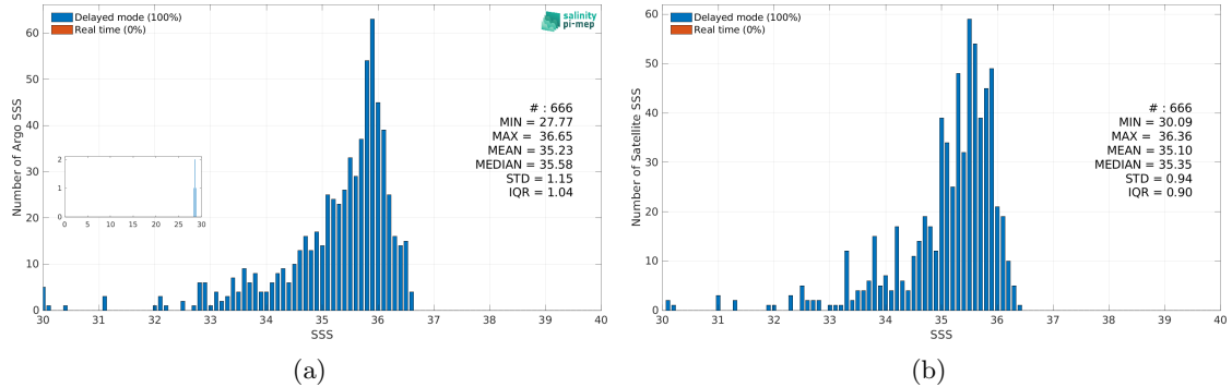
Figure 3: Histograms of SSS from Argo (a) and Aquarius SSS L3 OR v5 - Monthly - Rain mask (NASA-GSFC) (b) considering all match-up pairs per bins of 0.1 over the Congo river plume Pi-MEP region and for the full satellite product period.
