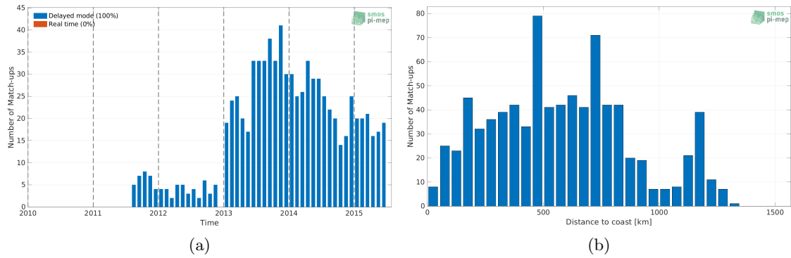
Figure 1: Number of match-ups between Argo and Aquarius SSS L3 OR v5 - Monthly - Rain mask (NASA-GSFC) SSS as a function of time (a) and as function of the distance to coast (b) over the Congo river plume Pi-MEP region and for the full satellite product period.
