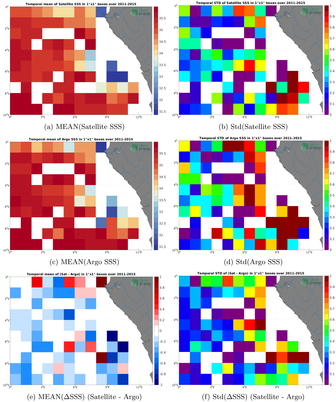
Figure 6: Temporal mean (left) and Std (right) of SSS from Aquarius SSS L3 OR v5 - Monthly - Rain mask (NASA-GSFC) (top), Argo (middle), and of \Delta SSS (Satellite - Argo). Only match-up pairs are used to generate these maps.
