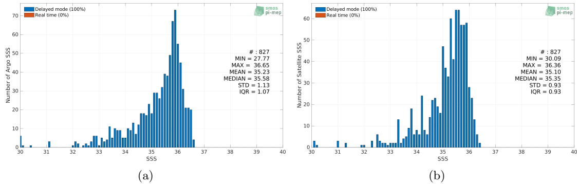
Figure 2: Histograms of SSS from Argo (a) and Aquarius SSS L3 OR v5 - Monthly - Rain mask (NASA-GSFC) (b) considering all match-up pairs per bins of 0.1 over the Congo river plume Pi-MEP region and for the full satellite product period.
