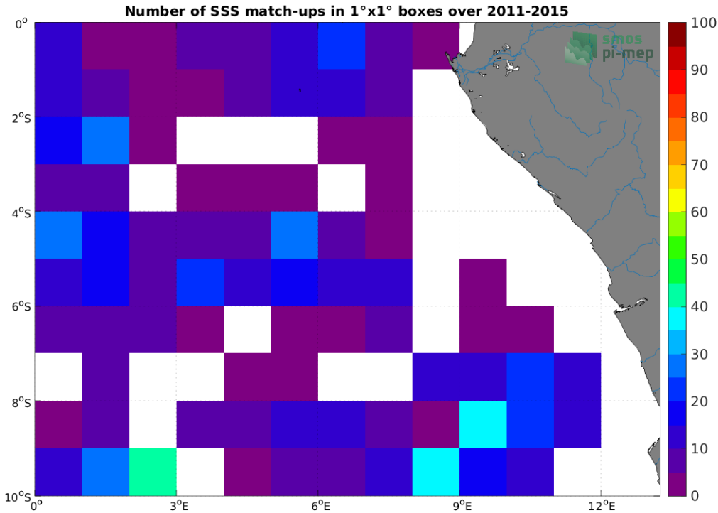
Figure 4: Number of SSS match-ups between Argo SSS and the Aquarius SSS L3 OR v5 - Monthly - Rain mask (NASA-GSFC) SSS product for the Congo river plume Pi-MEP region over 1°x1° boxes and for the full satellite product period.
