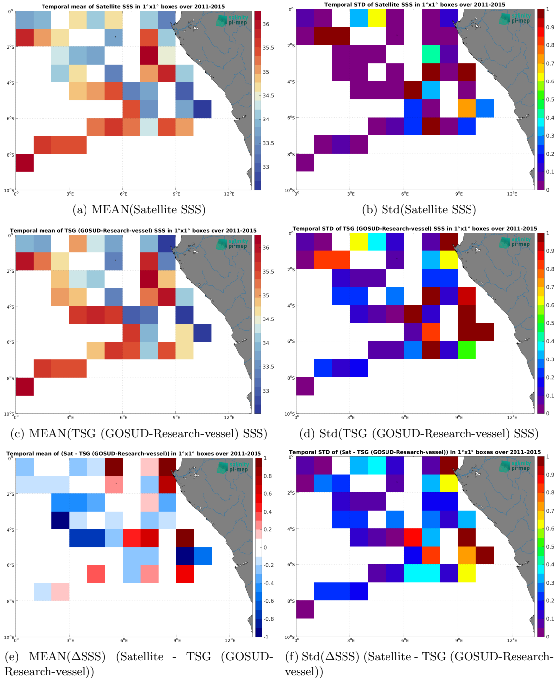
Figure 7: Temporal mean (left) and Std (right) of SSS from Aquarius SSS L3 CAP v5 - 7-Day running (JPL) (top), TSG (GOSUD-Research-vessel) (middle), and of \Delta SSS (Satellite - TSG (GOSUD-Research-vessel)). Only match-up pairs are used to generate these maps.
