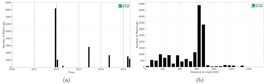
Figure 2: Number of match-ups between TSG (GOSUD-Research-vessel) and Aquarius SSS L3 CAP v5 - 7-Day running (JPL) SSS as a function of time (a) and as function of the distance to coast (b) over the Congo river plume Pi-MEP region and for the full satellite product period.
