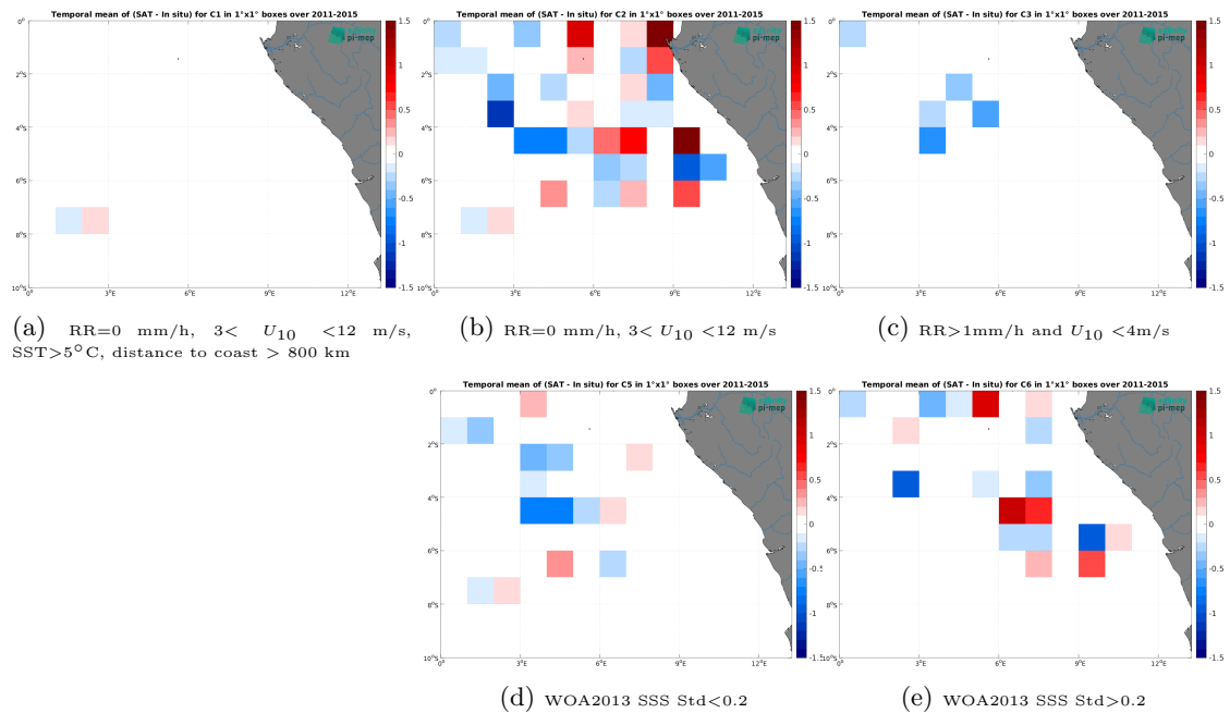
Figure 14: Temporal mean gridded over spatial boxes of size 1^\circ \times 1^\circ of \Delta SSS (Aquarius SSS L3 CAP v5 - 7-Day running (JPL) - TSG (GOSUD-Research-vessel)) for 5 different subdatasets corresponding to:RR=0 mm/h, 3 < U_{10} < 12 m/s, SST > 5^\circ\text{C} , distance to coast > 800 km (a), RR=0 mm/h, 3 < U_{10} < 12 m/s (b), RR > 1 mm/h and U_{10} < 4 m/s (c), WOA2013 SSS Std < 0.2 (d), WOA2013 SSS Std > 0.2 (e).
