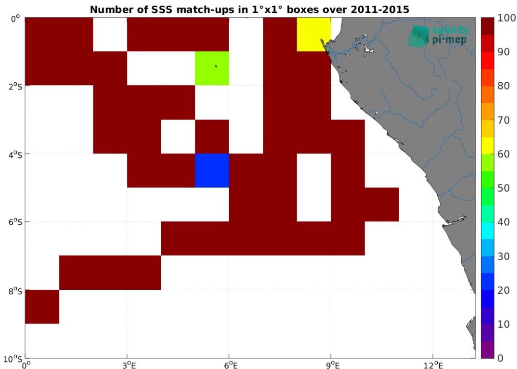
Figure 5: Number of SSS match-ups between TSG (GOSUD-Research-vessel) SSS and the Aquarius SSS L3 CAP v5 - 7-Day running (JPL) SSS product for the Congo river plume Pi-MEP region over 1^\circ \times 1^\circ boxes and for the full satellite product period.
