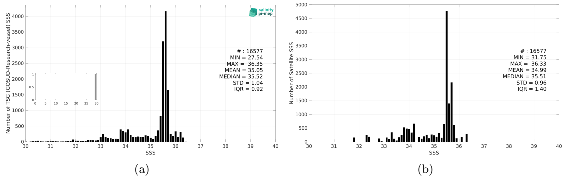
Figure 3: Histograms of SSS from TSG (GOSUD-Research-vessel) (a) and Aquarius SSS L3 CAP v5 - 7-Day running (JPL) (b) considering all match-up pairs per bins of 0.1 over the Congo river plume Pi-MEP region and for the full satellite product period.
