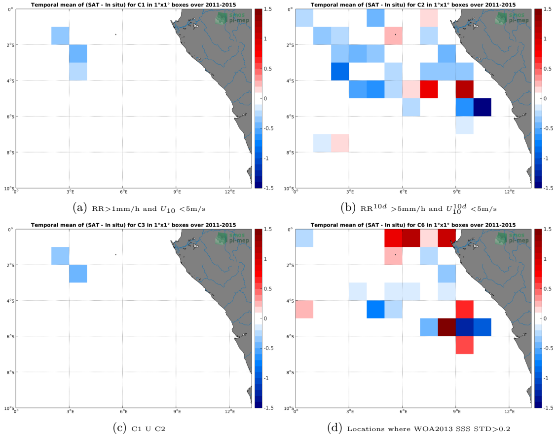
Figure 12: Temporal mean gridded over spatial boxes of size 1^\circ \times 1^\circ of \Delta SSS (Aquarius-L3-JPL-V5-7DAY-RUNNING - TSG-GOSUD-Research-vessel) for 4 different subdatasets corresponding to: RR > 1mm/h and U_{10} < 5m/s (a), RR 10d > 5mm/h and U_{10}^{10d} < 5m/s (b), C1 U C2 (c), Locations where WOA2013 SSS STD > 0.2 (d).
