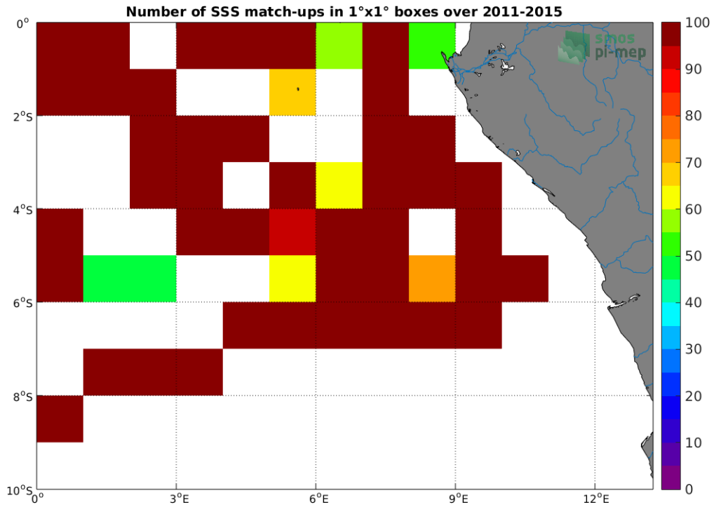
Figure 4: Number of SSS match-ups between TSG-GOSUD-Research-vessel SSS and the Aquarius-L3-JPL-V5-7DAY-RUNNING SSS product for the Congo river plume Pi-MEP region over 1°x1° boxes and for the full satellite product period.
