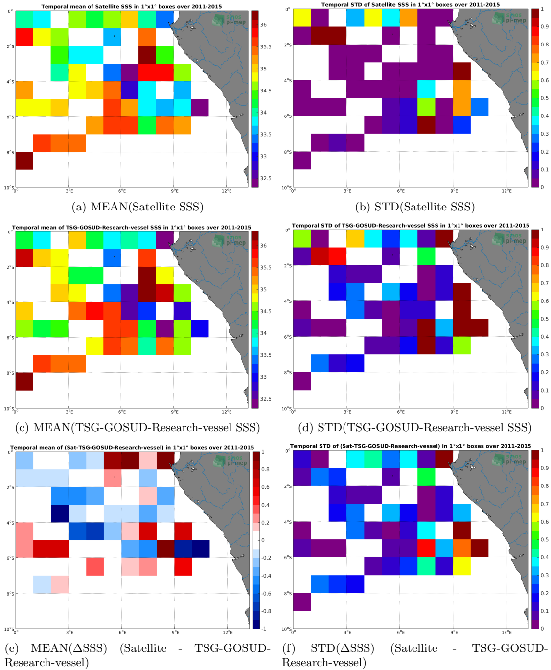
Figure 6: Temporal mean (left) and STD (right) of SSS from Aquarius-L3-JPL-V5-7DAY-RUNNING (top), TSG-GOSUD-Research-vessel (middle), and of \Delta SSS (Satellite - TSG-GOSUD-Research-vessel). Only match-up pairs are used to generate these maps.
