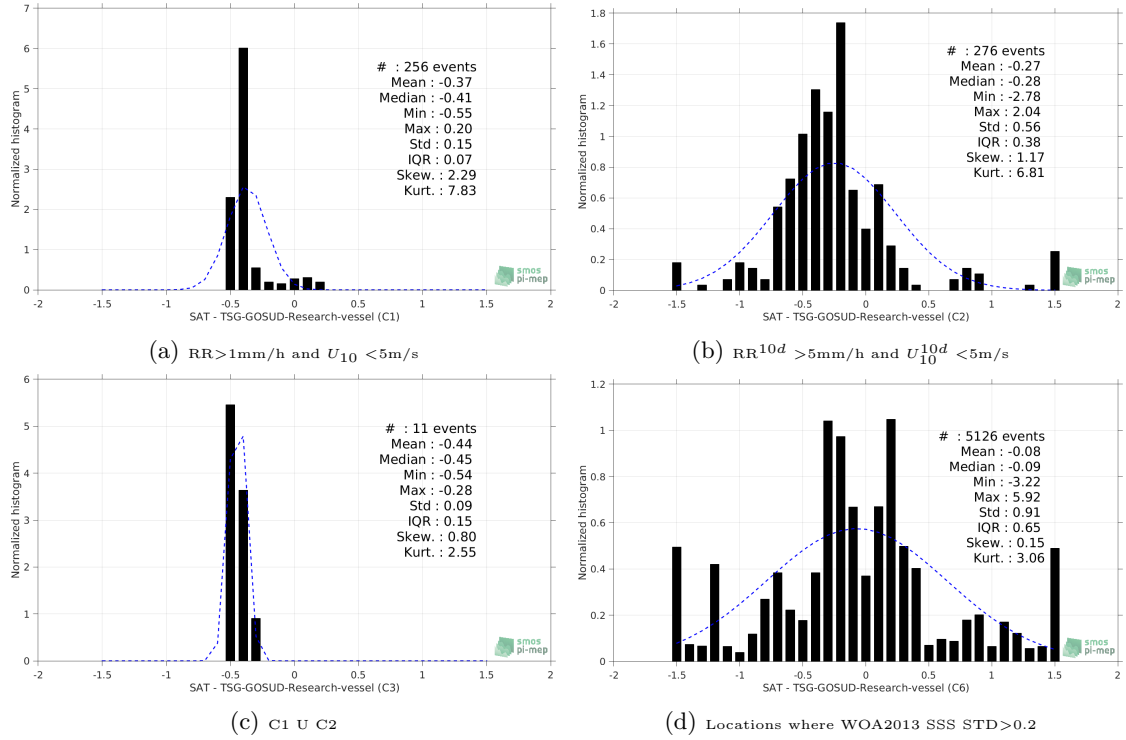
Figure 13: Normalized histogram of \Delta\text{SSS} (Aquarius-L3-JPL-V5-7DAY-RUNNING - TSG-GOSUD-Research-vessel) for 6 different subdatasets corresponding to: RR > 1mm/h and U_{10} < 5\text{m/s} (a), \text{RR}^{10d} > 5\text{mm/h} and U_{10}^{10d} < 5\text{m/s} (b), C1 U C2 (c), Locations where WOA2013 SSS STD > 0.2 (d).
