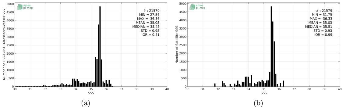
Figure 2: Histograms of SSS from TSG-GOSUD-Research-vessel (a) and Aquarius-L3-JPL-V5-7DAY-RUNNING (b) considering all match-up pairs per bins of 0.1 over the Congo river plume Pi-MEP region and for the full satellite product period.
