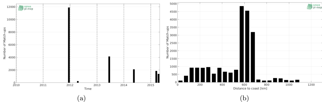
Figure 1: Number of match-ups between TSG-GOSUD-Research-vessel and Aquarius-L3-JPL-V5-7DAY-RUNNING SSS as a function of time (a) and as function of the distance to coast (b) over the Congo river plume Pi-MEP region and for the full satellite product period.
