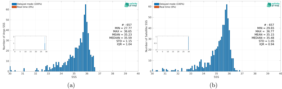
Figure 3: Histograms of SSS from Argo (a) and Aquarius SSS L3 CAP v5 - 7-Day running (JPL) (b) considering all match-up pairs per bins of 0.1 over the Congo river plume Pi-MEP region and for the full satellite product period.
