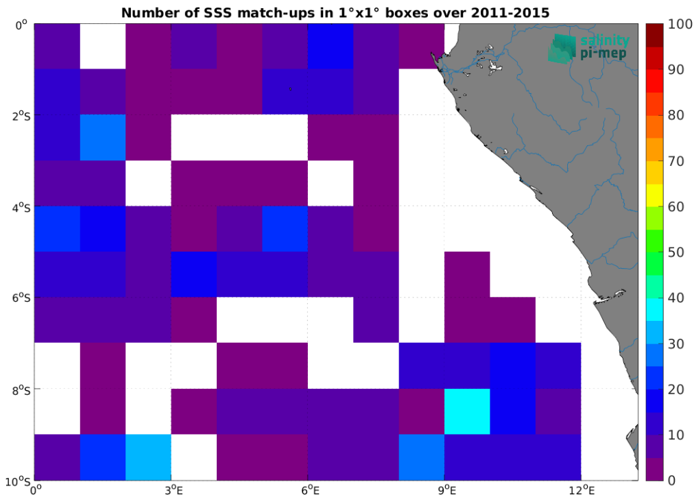
Figure 5: Number of SSS match-ups between Argo SSS and the Aquarius SSS L3 CAP v5 - 7-Day running (JPL) SSS product for the Congo river plume Pi-MEP region over 1^\circ \times 1^\circ boxes and for the full satellite product period.
