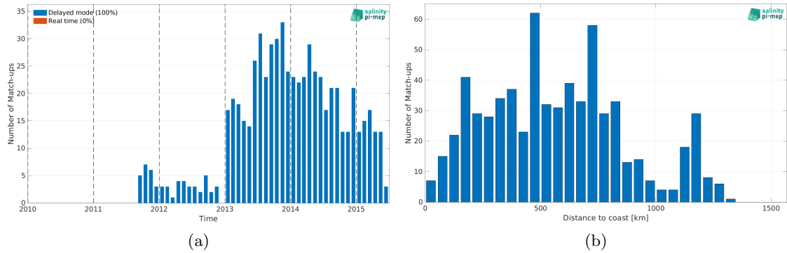
Figure 2: Number of match-ups between Argo and Aquarius SSS L3 CAP v5 - 7-Day running (JPL) SSS as a function of time (a) and as function of the distance to coast (b) over the Congo river plume Pi-MEP region and for the full satellite product period.
