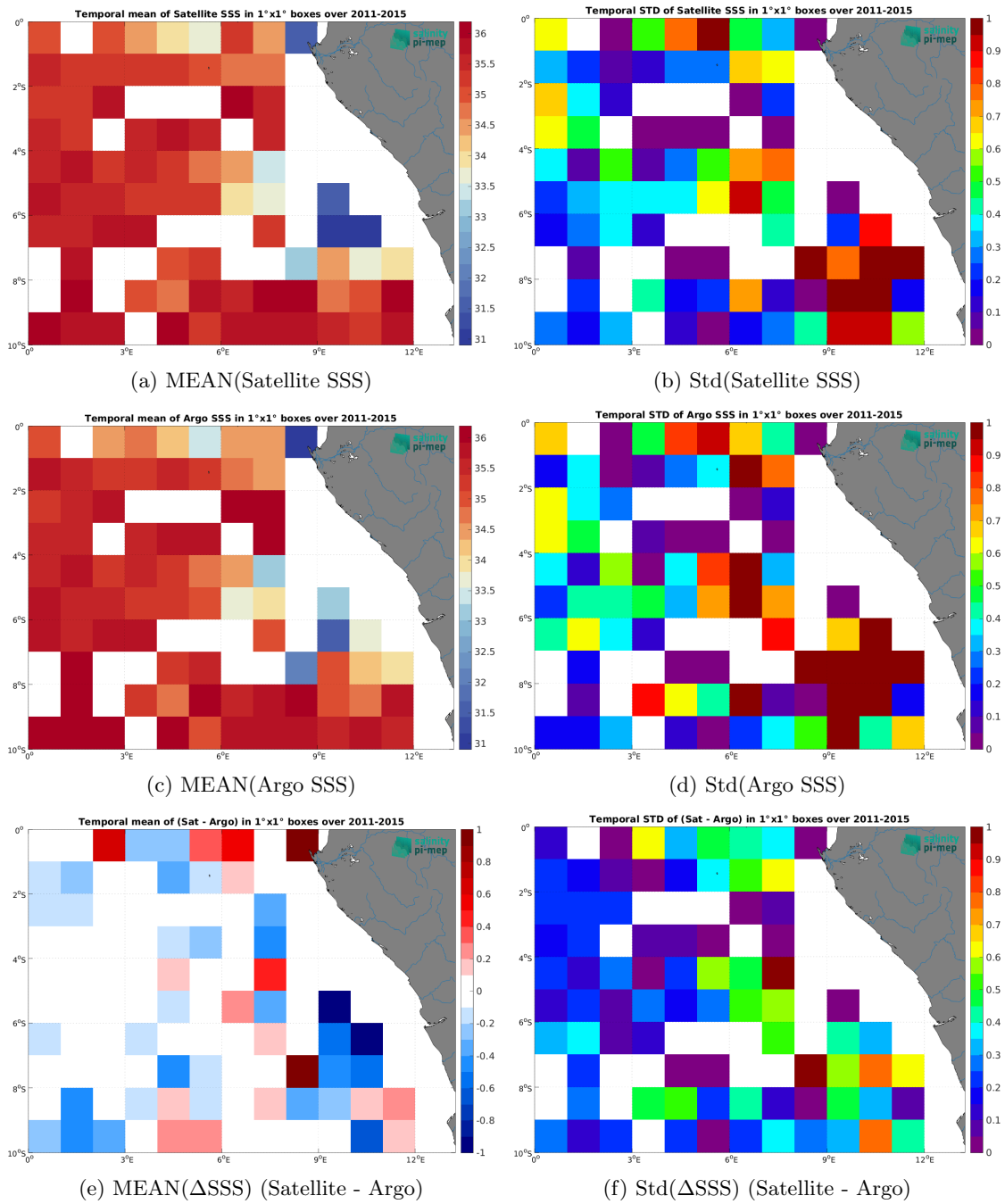
Figure 7: Temporal mean (left) and Std (right) of SSS from Aquarius SSS L3 CAP v5 - 7-Day running (JPL) (top), Argo (middle), and of \Delta SSS (Satellite - Argo). Only match-up pairs are used to generate these maps.
