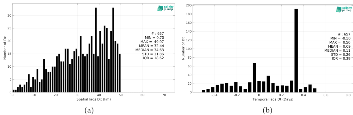
Figure 6: Histograms of the spatial (a) and temporal (b) lags between the location/time of the Argo measurement and the date of the corresponding Aquarius SSS L3 CAP v5 - 7-Day running (JPL) SSS pixel.
