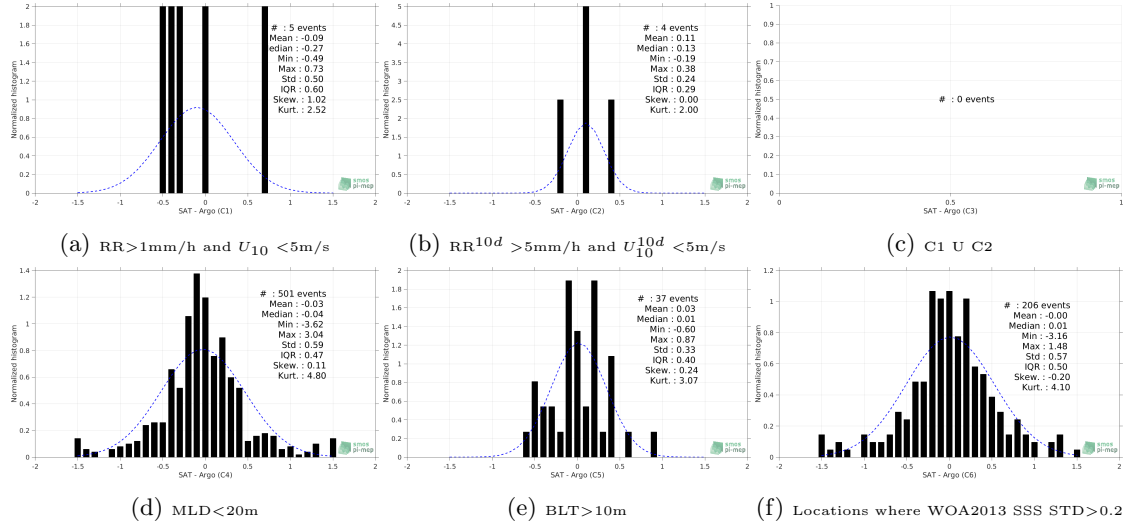
Figure 13: Normalized histogram of \Delta SSS (Aquarius-L3-JPL-V5-7DAY-RUNNING - Argo) for 6 different subdatasets corresponding to: RR > 1\text{mm/h} and U_{10} < 5\text{m/s} (a), RR^{10d} > 5\text{mm/h} and U_{10}^{10d} < 5\text{m/s} (b), C1 U C2 (c), MLD < 20\text{m} (d), BLT > 10\text{m} (e), Locations where WOA2013 SSS STD > 0.2 (f).
