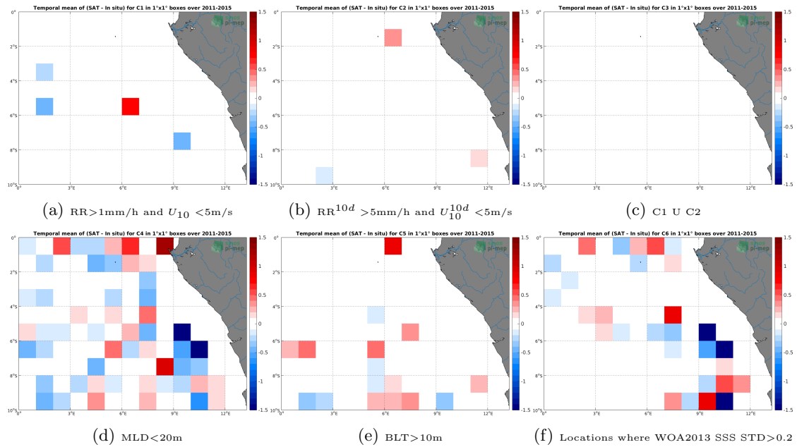
Figure 12: Temporal mean gridded over spatial boxes of size 1^\circ \times 1^\circ of \Delta SSS (Aquarius-L3-JPL-V5-7DAY-RUNNING - Argo) for 6 different subdatasets corresponding to: RR > 1\text{mm/h} and U_{10} < 5\text{m/s} (a), RR^{10d} > 5\text{mm/h} and U_{10}^{10d} < 5\text{m/s} (b), C1 U C2 (c), MLD < 20\text{m} (d), BLT > 10\text{m} (e), Locations where WOA2013 SSS STD > 0.2 (f).
