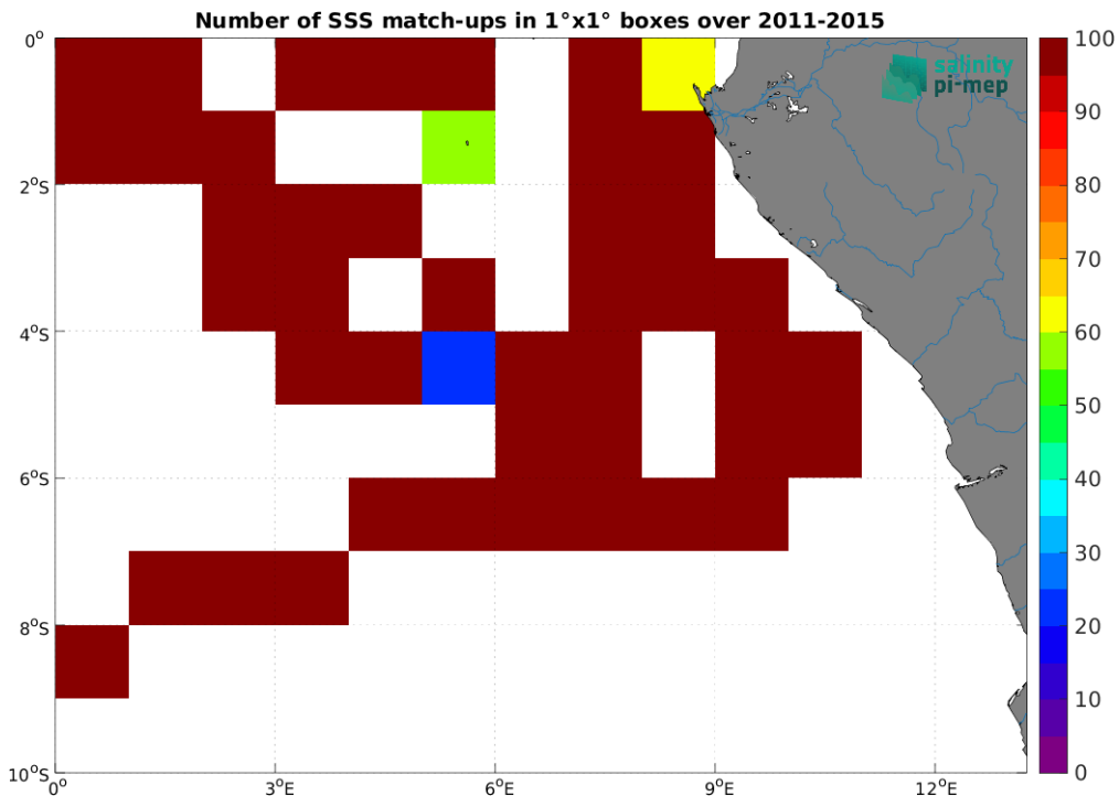
Figure 5: Number of SSS match-ups between TSG (GOSUD-Research-vessel) SSS and the Aquarius SSS L3 CAP v5 - Monthly (JPL) SSS product for the Congo river plume Pi-MEP region over 1^\circ \times 1^\circ boxes and for the full satellite product period.
