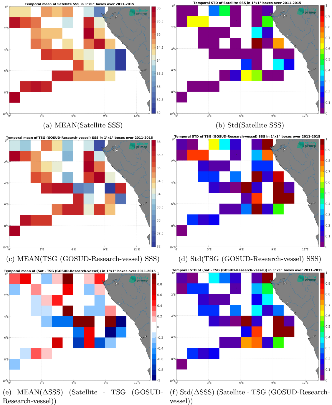
Figure 7: Temporal mean (left) and Std (right) of SSS from Aquarius SSS L3 CAP v5 - Monthly (JPL) (top), TSG (GOSUD-Research-vessel) (middle), and of \Delta SSS (Satellite - TSG (GOSUD-Research-vessel)). Only match-up pairs are used to generate these maps.
