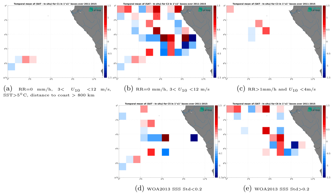
Figure 14: Temporal mean gridded over spatial boxes of size 1^\circ \times 1^\circ of \Delta SSS (Aquarius SSS L3 CAP v5 - Monthly (JPL) - TSG (GOSUD-Research-vessel)) for 5 different subdatasets corresponding to:RR=0 mm/h, 3 < U_{10} < 12 m/s, SST > 5°C, distance to coast > 800 km (a), RR=0 mm/h, 3 < U_{10} < 12 m/s (b), RR > 1mm/h and U_{10} < 4 m/s (c), WOA2013 SSS Std < 0.2 (d), WOA2013 SSS Std > 0.2 (e).
