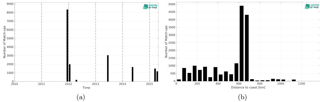
Figure 2: Number of match-ups between TSG (GOSUD-Research-vessel) and Aquarius SSS L3 CAP v5 - Monthly (JPL) SSS as a function of time (a) and as function of the distance to coast (b) over the Congo river plume Pi-MEP region and for the full satellite product period.
