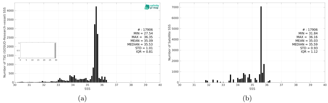
Figure 3: Histograms of SSS from TSG (GOSUD-Research-vessel) (a) and Aquarius SSS L3 CAP v5 - Monthly (JPL) (b) considering all match-up pairs per bins of 0.1 over the Congo river plume Pi-MEP region and for the full satellite product period.
