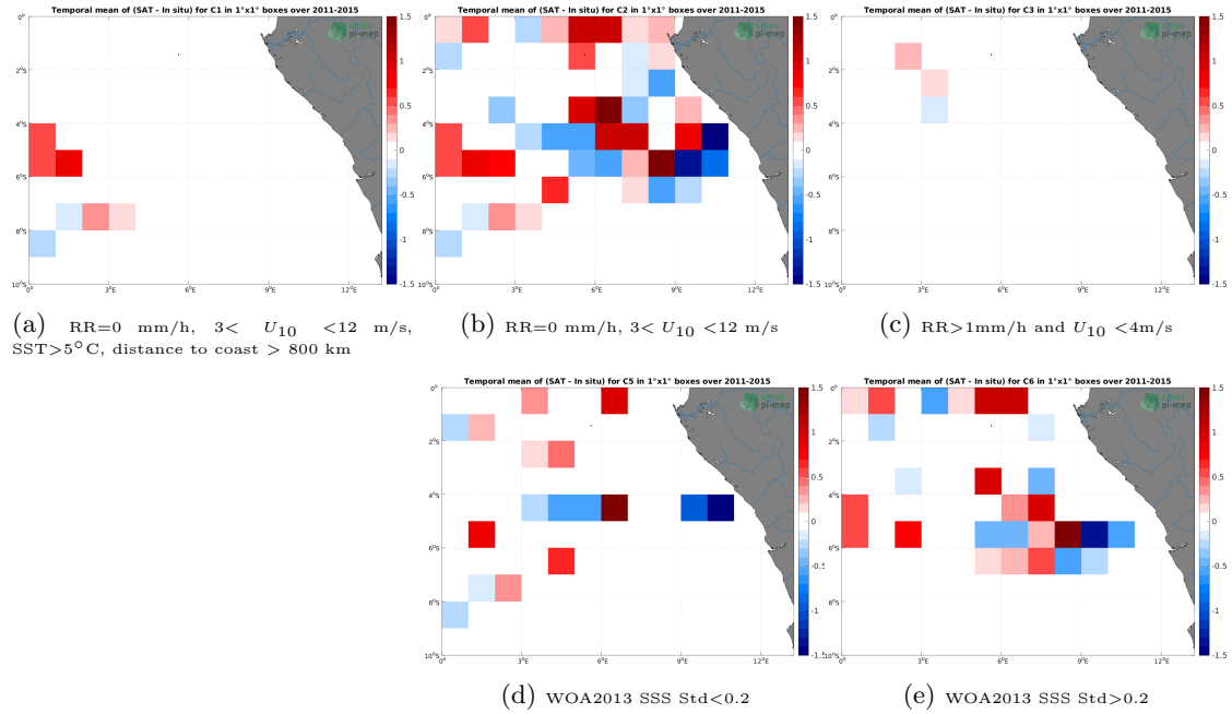
Figure 12: Temporal mean gridded over spatial boxes of size 1^{\circ}\times 1^{\circ} of \Delta SSS (Aquarius SSS L3 CAP v5 - Monthly (JPL) - TSG (GOSUD-Research-vessel)) for 5 different subdatasets corresponding to:RR=0 mm/h, 3 < U_{10} < 12 m/s, SST >5^{\circ}\text{C} , distance to coast > 800 km (a), RR=0 mm/h, 3 < U_{10} < 12 m/s (b), RR >1 mm/h and U_{10} < 4 m/s (c), WOA2013 SSS Std <0.2 (d), WOA2013 SSS Std >0.2 (e).
