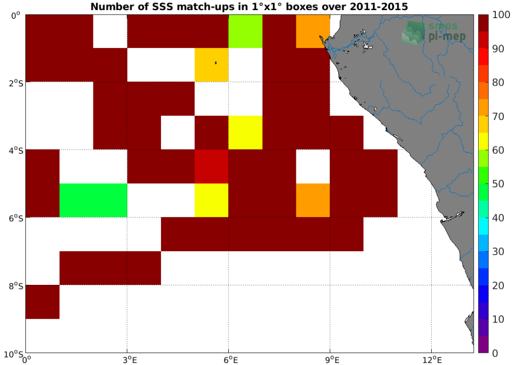
Figure 4: Number of SSS match-ups between TSG (GOSUD-Research-vessel) SSS and the Aquarius SSS L3 CAP v5 - Monthly (JPL) SSS product for the Congo river plume Pi-MEP region over 1^\circ \times 1^\circ boxes and for the full satellite product period.
