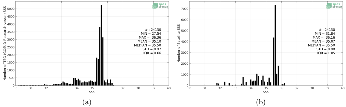
Figure 2: Histograms of SSS from TSG (GOSUD-Research-vessel) (a) and Aquarius SSS L3 CAP v5 - Monthly (JPL) (b) considering all match-up pairs per bins of 0.1 over the Congo river plume Pi-MEP region and for the full satellite product period.
