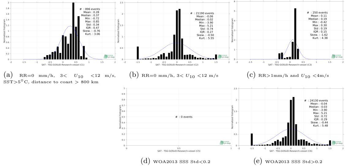
Figure 13: Normalized histogram of \Delta SSS (Aquarius-L3-JPL-V5-MONTHLY - TSG-GOSUD-Research-vessel) for 5 different subdatasets corresponding to: RR=0 mm/h, 3 < U_{10} < 12 m/s, SST>5°C, distance to coast > 800 km (a), RR=0 mm/h, 3 < U_{10} < 12 m/s (b), RR>1mm/h and U_{10} < 4 m/s (c), WOA2013 SSS Std<0.2 (d), WOA2013 SSS Std>0.2 (e).
