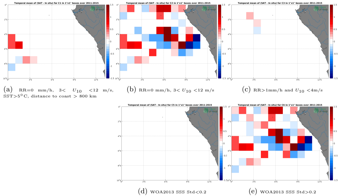
Figure 12: Temporal mean gridded over spatial boxes of size 1^\circ \times 1^\circ of \Delta SSS (Aquarius-L3-JPL-V5-MONTHLY - TSG-GOSUD-Research-vessel) for 5 different subdatasets corresponding to: RR=0 mm/h, 3 < U_{10} < 12 m/s, SST >5^\circ C, distance to coast > 800 km (a), RR=0 mm/h, 3 < U_{10} < 12 m/s (b), RR >1 mm/h and U_{10} < 4 m/s (c), WOA2013 SSS Std <0.2 (d), WOA2013 SSS Std >0.2 (e).
