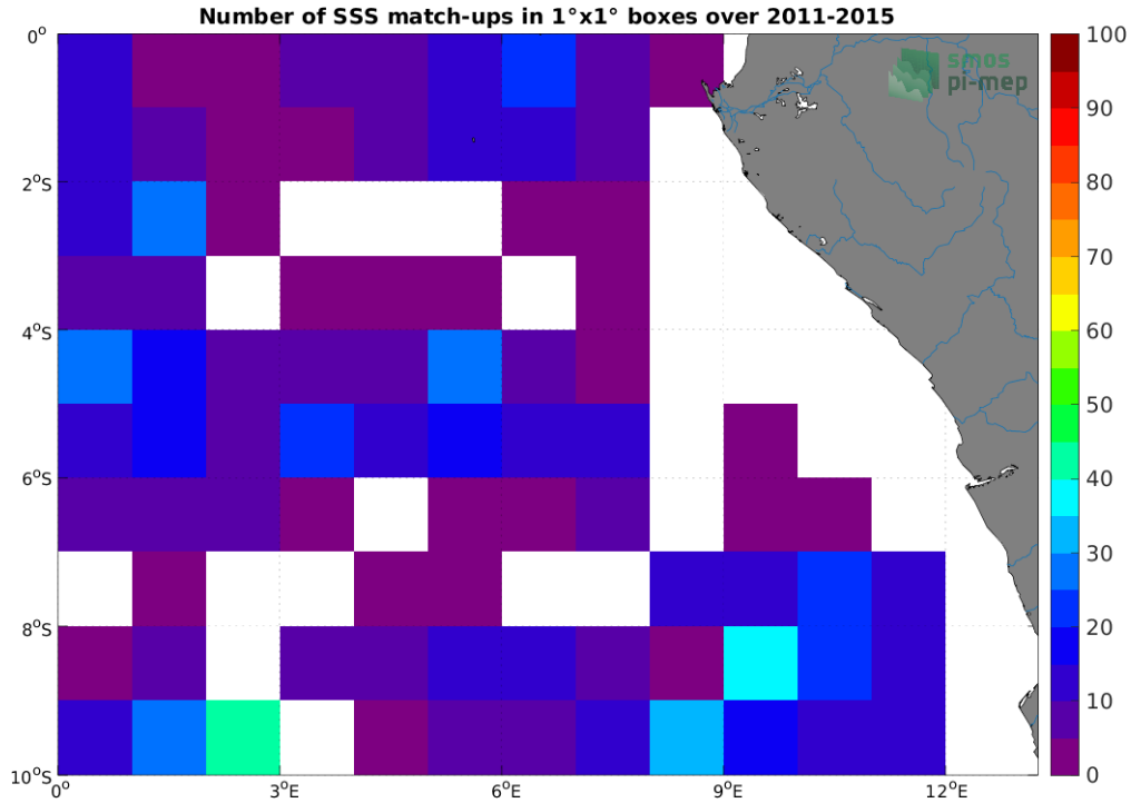
Figure 4: Number of SSS match-ups between Argo SSS and the Aquarius SSS L3 CAP v5 - Monthly (JPL) SSS product for the Congo river plume Pi-MEP region over 1^\circ \times 1^\circ boxes and for the full satellite product period.
