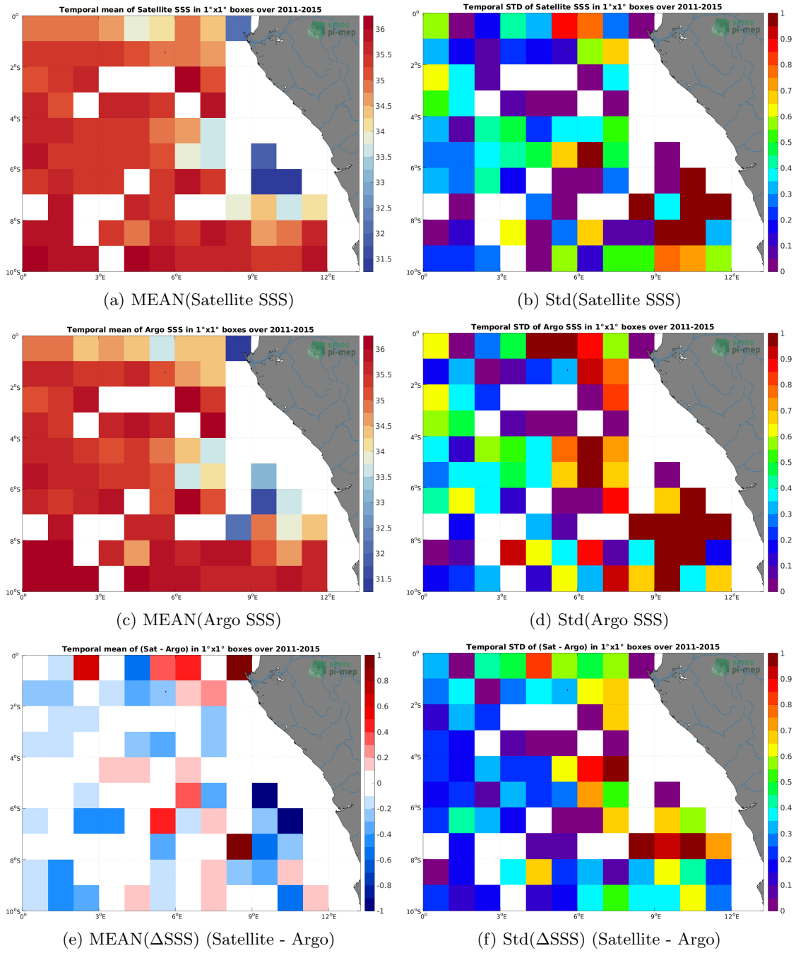
Figure 6: Temporal mean (left) and Std (right) of SSS from Aquarius SSS L3 CAP v5 - Monthly (JPL) (top), Argo (middle), and of \Delta SSS (Satellite - Argo). Only match-up pairs are used to generate these maps.
