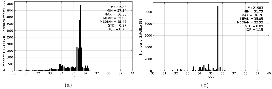
Figure 2: Histograms of SSS from TSG-GOSUD-Research-vessel (a) and Aquarius-L3-JPL-V4-MONTHLY (b) considering all match-up pairs per bins of 0.1 over the Congo river plume Pi-MEP region and for the full satellite product period.
