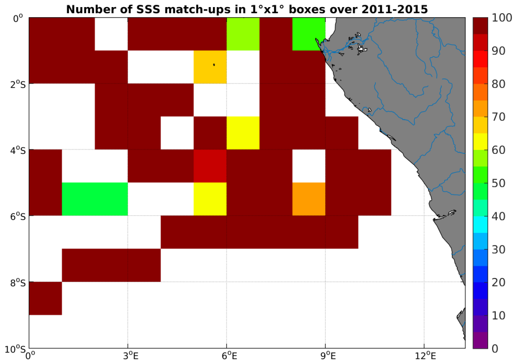
Figure 4: Number of SSS match-ups between TSG-GOSUD-Research-vessel SSS and the Aquarius-L3-JPL-V4-MONTHLY SSS product for the Congo river plume Pi-MEP region over 1^\circ \times 1^\circ boxes and for the full satellite product period.
