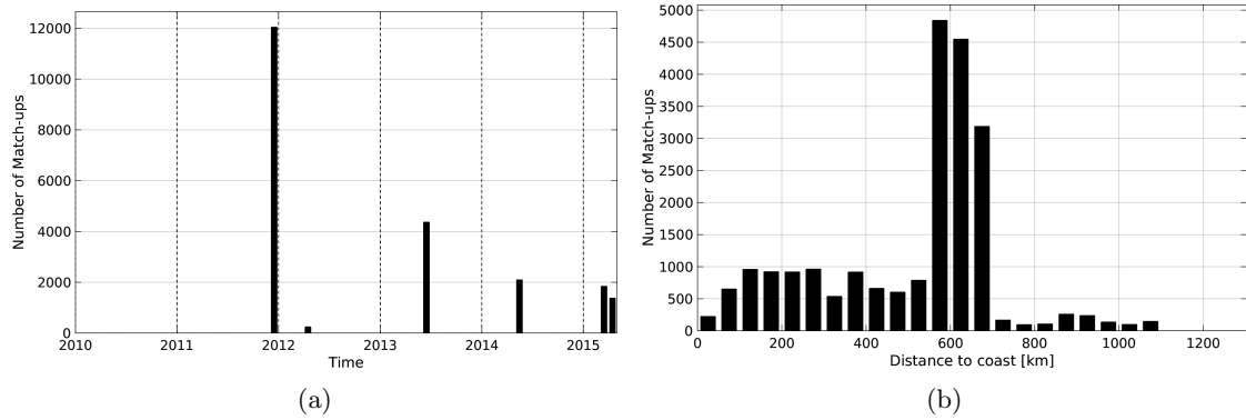
Figure 1: Number of match-ups between TSG-GOSUD-Research-vessel and Aquarius-L3-JPL-V4-MONTHLY SSS as a function of time (a) and as function of the distance to coast (b) over the Congo river plume Pi-MEP region and for the full satellite product period.
