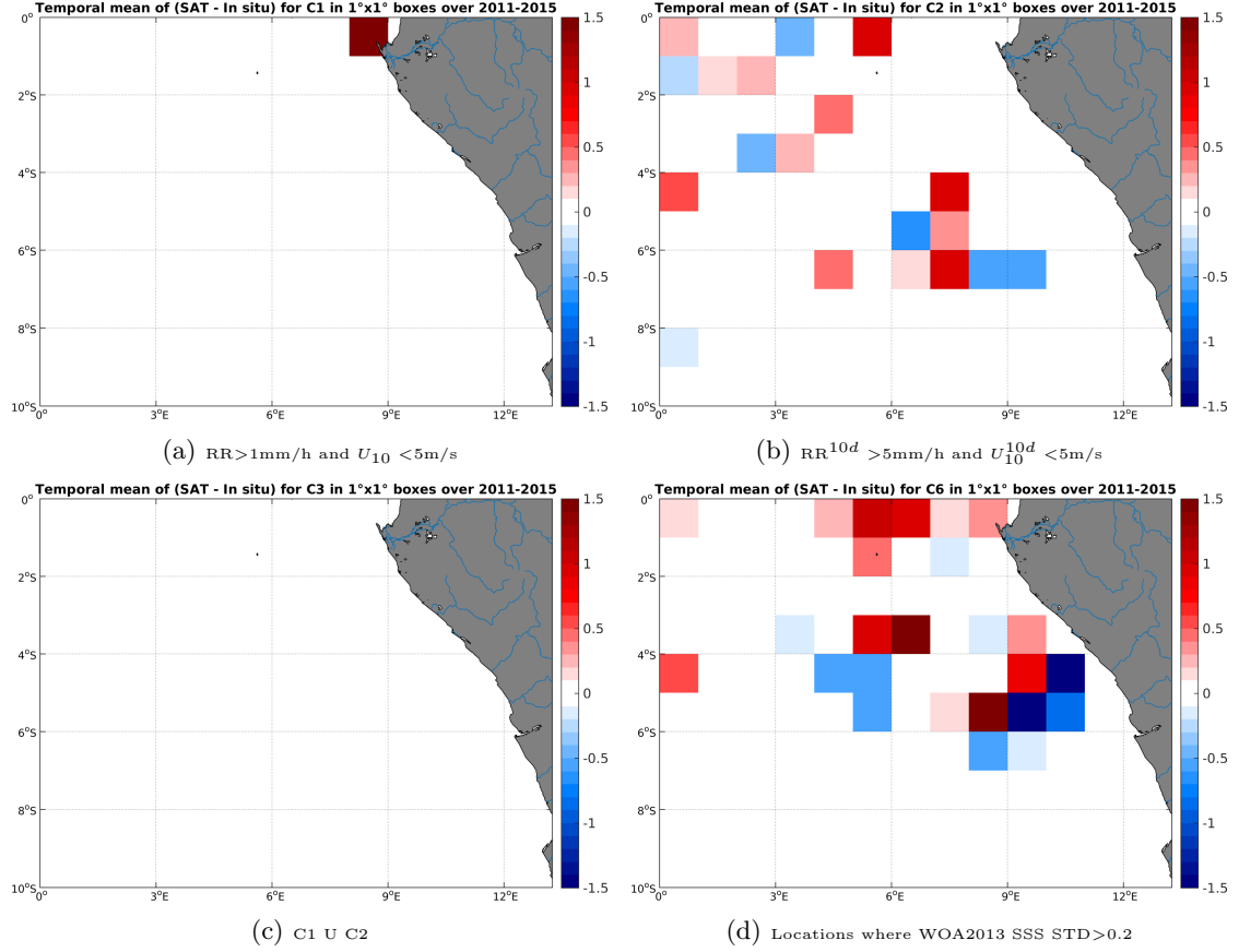
Figure 12: Temporal mean gridded over spatial boxes of size 1^\circ \times 1^\circ of \Delta SSS (Aquarius-L3-JPL-V4-MONTHLY - TSG-GOSUD-Research-vessel) for 4 different subdatasets corresponding to: RR > 1 mm/h and U_{10} < 5 m/s (a), RR^{10d} > 5 mm/h and U_{10}^{10d} < 5 m/s (b), C1 U C2 (c), Locations where WOA2013 SSS STD > 0.2 (d).
