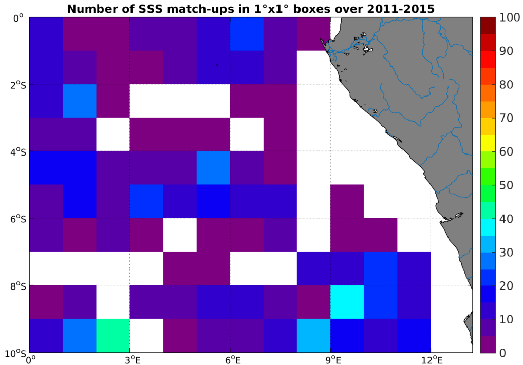
Figure 4: Number of SSS match-ups between Argo SSS and the Aquarius-L3-JPL-V4-MONTHLY SSS product for the Congo river plume Pi-MEP region over 1^\circ \times 1^\circ boxes and for the full satellite product period.
