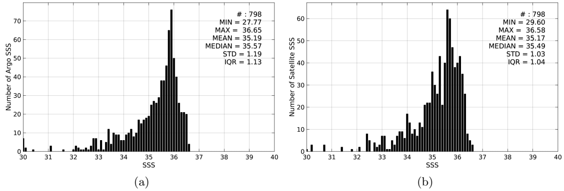
Figure 2: Histograms of SSS from Argo (a) and Aquarius-L3-JPL-V4-MONTHLY (b) considering all match-up pairs per bins of 0.1 over the Congo river plume Pi-MEP region and for the full satellite product period.
