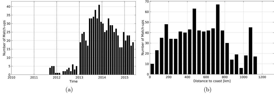
Figure 1: Number of match-ups between Argo and Aquarius-L3-JPL-V4-MONTHLY SSS as a function of time (a) and as function of the distance to coast (b) over the Congo river plume Pi-MEP region and for the full satellite product period.
