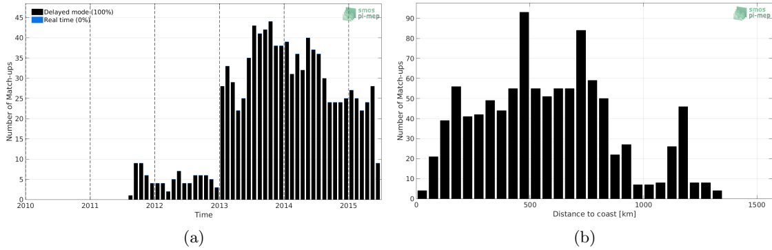
Figure 1: Number of match-ups between Argo and Aquarius SSS L2-AVERAGED OR v5 (NASA-GSFC) SSS as a function of time (a) and as function of the distance to coast (b) over the Congo river plume Pi-MEP region and for the full satellite product period.
