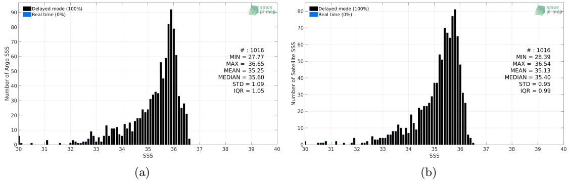
Figure 2: Histograms of SSS from Argo (a) and Aquarius SSS L2-AVERAGED OR v5 (NASA-GSFC) (b) considering all match-up pairs per bins of 0.1 over the Congo river plume Pi-MEP region and for the full satellite product period.
