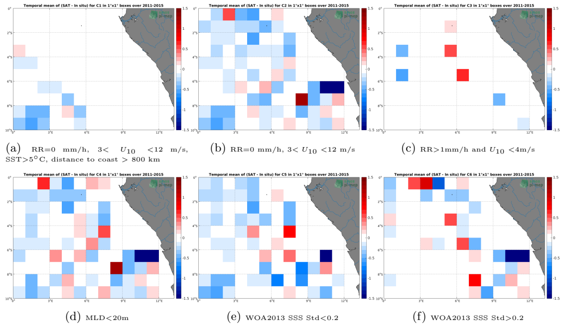
Figure 12: Temporal mean gridded over spatial boxes of size 1^\circ \times 1^\circ of \Delta SSS (Aquarius SSS L2-AVERAGED OR v5 (NASA-GSFC) - Argo) for 6 different subdatasets corresponding to:RR=0 mm/h, 3 < U_{10} < 12 m/s, SST >5^\circ C, distance to coast > 800 km (a), RR=0 mm/h, 3 < U_{10} < 12 m/s (b), RR >1 mm/h and U_{10} < 4 m/s (c),MLD <20 m (d),WOA2013 SSS Std <0.2 (e),WOA2013 SSS Std >0.2 (f).
