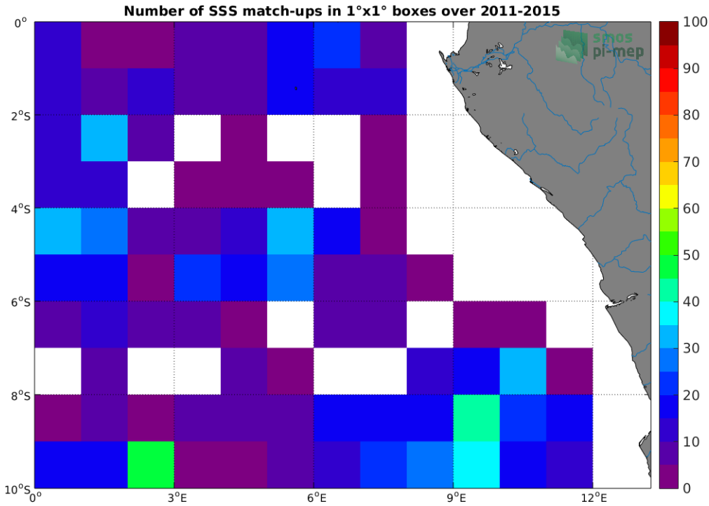
Figure 4: Number of SSS match-ups between Argo SSS and the Aquarius SSS L2-AVERAGED OR v5 (NASA-GSFC) SSS product for the Congo river plume Pi-MEP region over 1^{\circ} \times 1^{\circ} boxes and for the full satellite product period.
