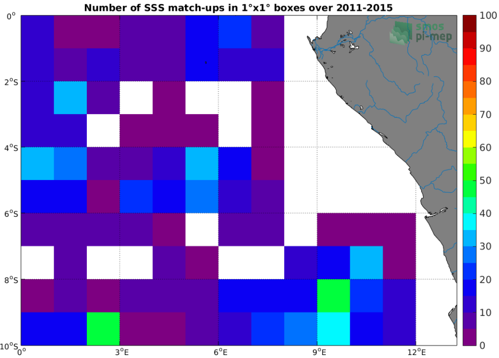
Figure 4: Number of SSS match-ups between Argo SSS and the Aquarius SSS L2-AVERAGED CAP v5 (JPL) SSS product for the Congo river plume Pi-MEP region over 1^\circ \times 1^\circ boxes and for the full satellite product period.
