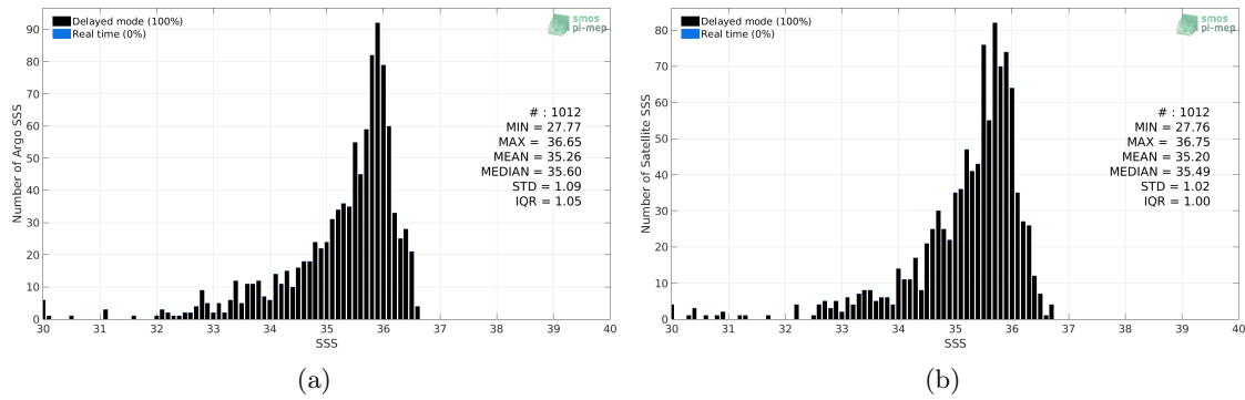
Figure 2: Histograms of SSS from Argo (a) and Aquarius SSS L2-AVERAGED CAP v5 (JPL) (b) considering all match-up pairs per bins of 0.1 over the Congo river plume Pi-MEP region and for the full satellite product period.
