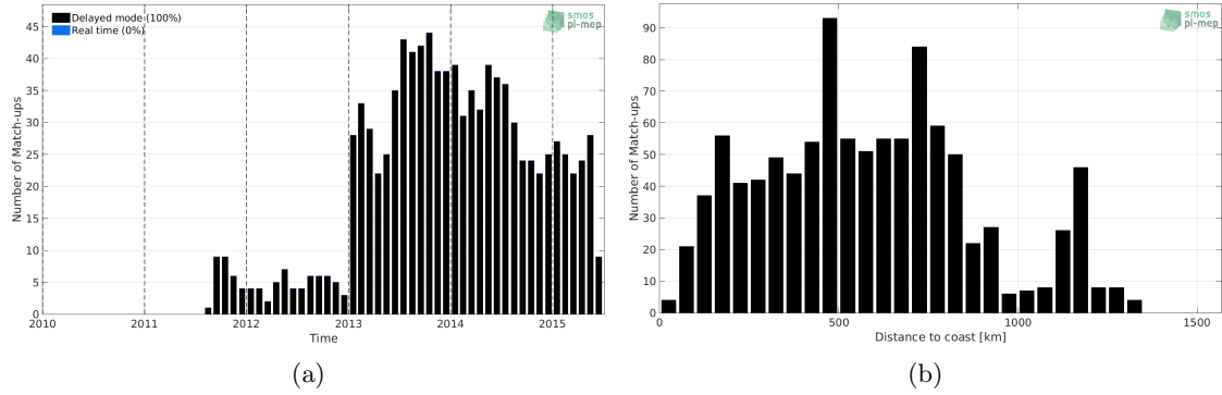
Figure 1: Number of match-ups between Argo and Aquarius SSS L2-AVERAGED CAP v5 (JPL) SSS as a function of time (a) and as function of the distance to coast (b) over the Congo river plume Pi-MEP region and for the full satellite product period.
