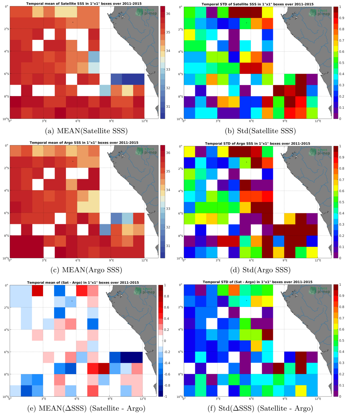
Figure 6: Temporal mean (left) and Std (right) of SSS from Aquarius SSS L2-AVERAGED CAP v5 (JPL) (top), Argo (middle), and of \Delta SSS (Satellite - Argo). Only match-up pairs are used to generate these maps.
