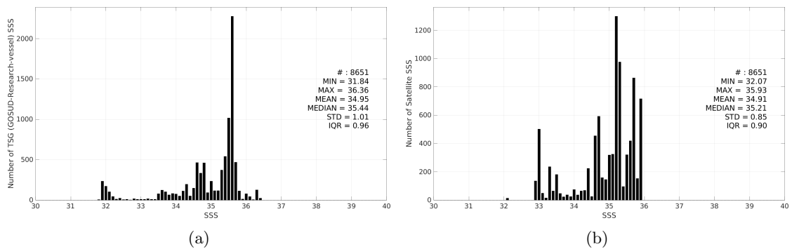
Figure 3: Histograms of SSS from TSG (GOSUD-Research-vessel) (a) and Aquarius SSS L2 OR v5 (NASA-GSFC) (b) considering all match-up pairs per bins of 0.1 over the Congo river plume Pi-MEP region and for the full satellite product period.
