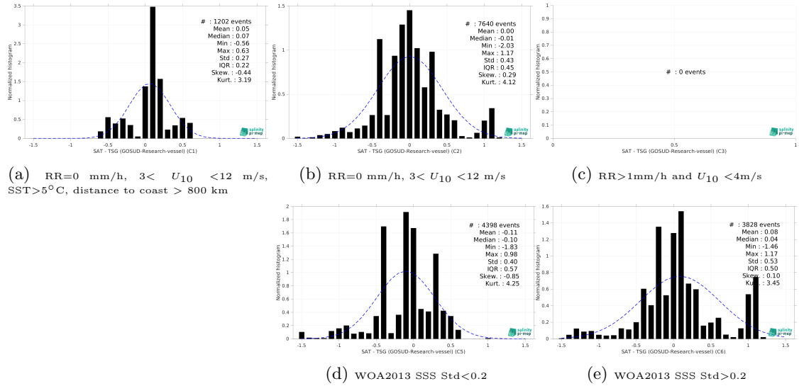
Figure 15: Normalized histogram of \Delta SSS (Aquarius SSS L2 OR v5 (NASA-GSFC) - TSG (GOSUD-Research-vessel)) for 5 different subdatasets corresponding to: RR=0 mm/h, 3 < U_{10} < 12 m/s, SST > 5°C, distance to coast > 800 km (a), RR=0 mm/h, 3 < U_{10} < 12 m/s (b), RR > 1mm/h and U_{10} < 4 m/s (c), WOA2013 SSS Std < 0.2 (d), WOA2013 SSS Std > 0.2 (e).
