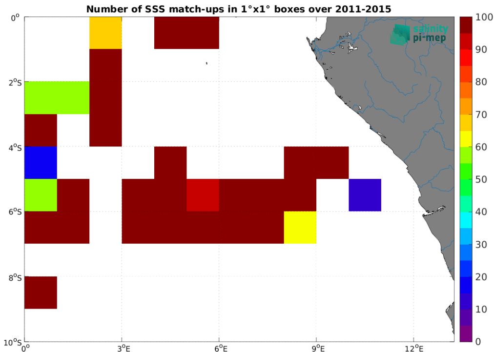
Figure 5: Number of SSS match-ups between TSG (GOSUD-Research-vessel) SSS and the Aquarius SSS L2 OR v5 (NASA-GSFC) SSS product for the Congo river plume Pi-MEP region over 1^\circ \times 1^\circ boxes and for the full satellite product period.
