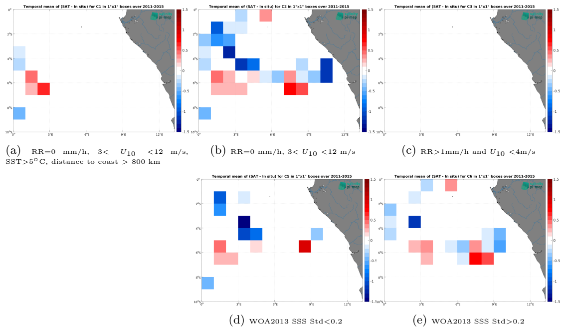
Figure 14: Temporal mean gridded over spatial boxes of size 1^\circ \times 1^\circ of \Delta SSS (Aquarius SSS L2 OR v5 (NASA-GSFC) - TSG (GOSUD-Research-vessel)) for 5 different subdatasets corresponding to:RR=0 mm/h, 3 < U_{10} < 12 m/s, SST>5°C, distance to coast > 800 km (a), RR=0 mm/h, 3 < U_{10} < 12 m/s (b), RR>1mm/h and U_{10} < 4 m/s (c), WOA2013 SSS Std<0.2 (d), WOA2013 SSS Std>0.2 (e).
