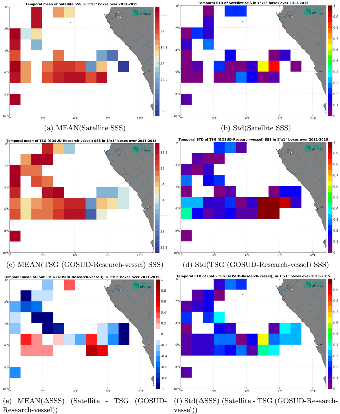
Figure 7: Temporal mean (left) and Std (right) of SSS from Aquarius SSS L2 OR v5 (NASA-GSFC) (top), TSG (GOSUD-Research-vessel) (middle), and of \Delta SSS (Satellite - TSG (GOSUD-Research-vessel)). Only match-up pairs are used to generate these maps.
