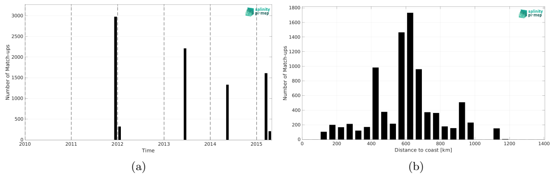
Figure 2: Number of match-ups between TSG (GOSUD-Research-vessel) and Aquarius SSS L2 OR v5 (NASA-GSFC) SSS as a function of time (a) and as function of the distance to coast (b) over the Congo river plume Pi-MEP region and for the full satellite product period.
