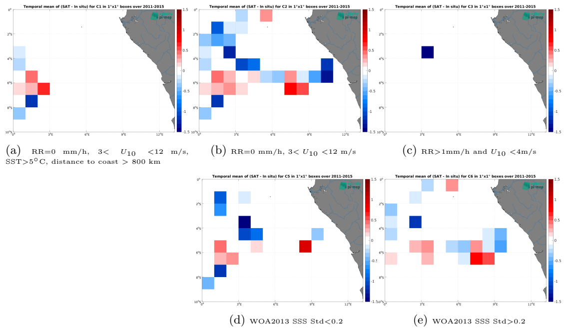
Figure 12: Temporal mean gridded over spatial boxes of size 1^\circ \times 1^\circ of \Delta SSS (Aquarius SSS L2 OR v5 (NASA-GSFC) - TSG (GOSUD-Research-vessel)) for 5 different subdatasets corresponding to: RR=0 mm/h, 3 < U_{10} < 12 m/s, SST > 5°C, distance to coast > 800 km (a), RR=0 mm/h, 3 < U_{10} < 12 m/s (b), RR > 1mm/h and U_{10} < 4 m/s (c), WOA2013 SSS Std < 0.2 (d), WOA2013 SSS Std > 0.2 (e).
