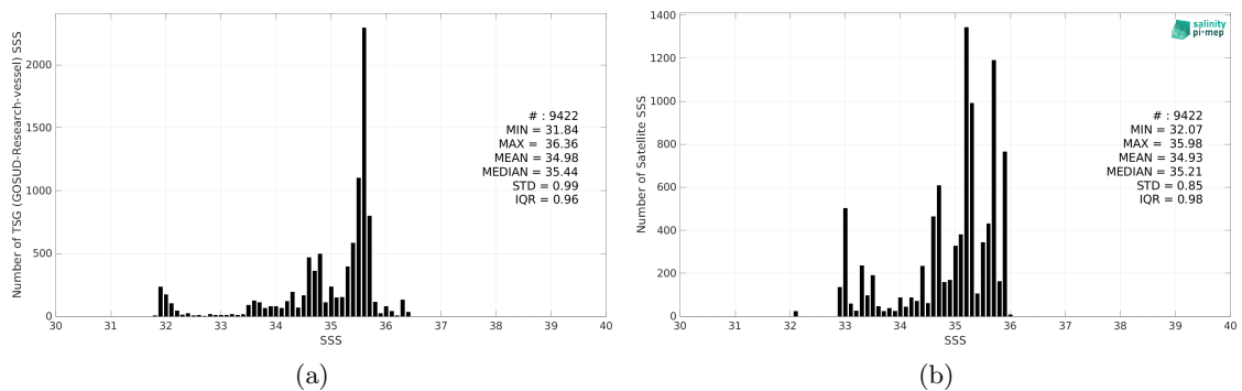
Figure 2: Histograms of SSS from TSG (GOSUD-Research-vessel) (a) and Aquarius SSS L2 OR v5 (NASA-GSFC) (b) considering all match-up pairs per bins of 0.1 over the Congo river plume Pi-MEP region and for the full satellite product period.
