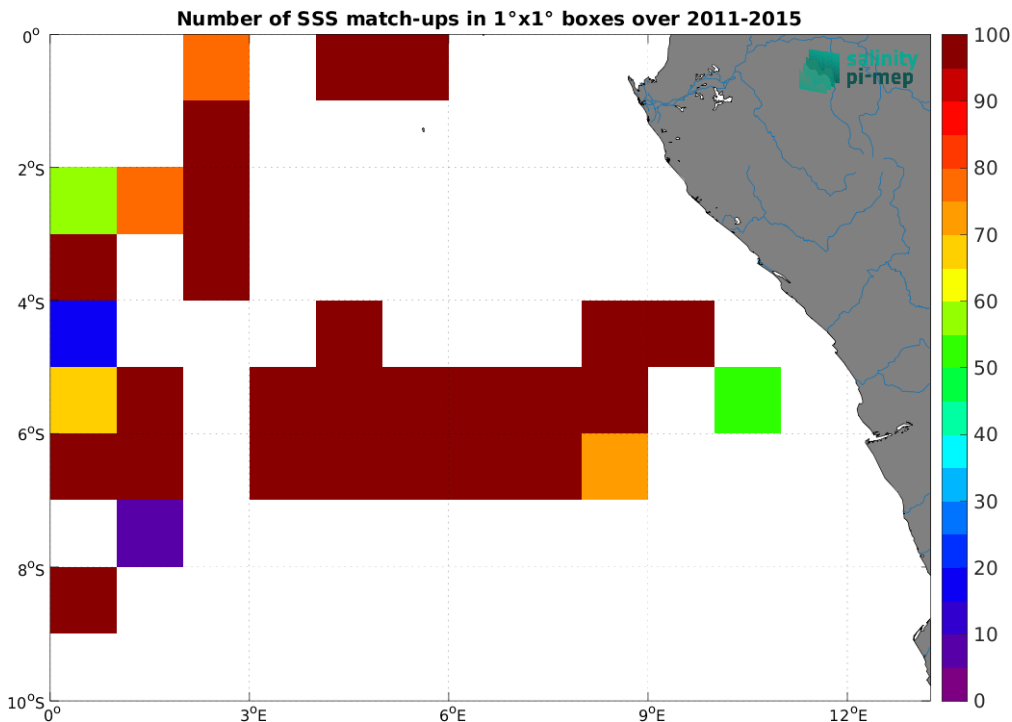
Figure 4: Number of SSS match-ups between TSG (GOSUD-Research-vessel) SSS and the Aquarius SSS L2 OR v5 (NASA-GSFC) SSS product for the Congo river plume Pi-MEP region over 1^\circ \times 1^\circ boxes and for the full satellite product period.
