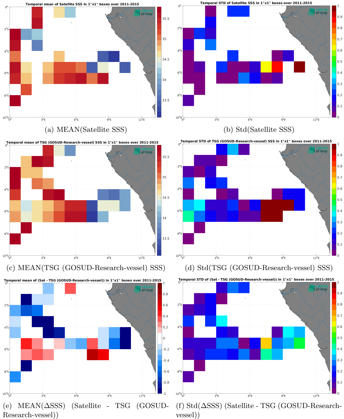
Figure 6: Temporal mean (left) and Std (right) of SSS from Aquarius SSS L2 OR v5 (NASA-GSFC) (top), TSG (GOSUD-Research-vessel) (middle), and of \Delta SSS (Satellite - TSG (GOSUD-Research-vessel)). Only match-up pairs are used to generate these maps.
