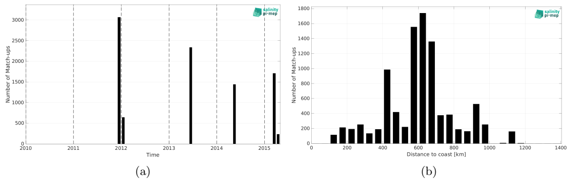
Figure 1: Number of match-ups between TSG (GOSUD-Research-vessel) and Aquarius SSS L2 OR v5 (NASA-GSFC) SSS as a function of time (a) and as function of the distance to coast (b) over the Congo river plume Pi-MEP region and for the full satellite product period.
