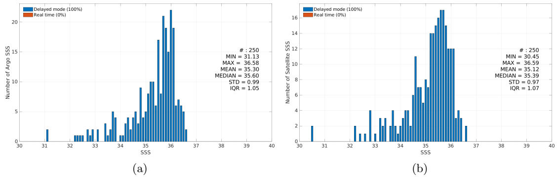
Figure 3: Histograms of SSS from Argo (a) and Aquarius SSS L2 OR v5 (NASA-GSFC) (b) considering all match-up pairs per bins of 0.1 over the Congo river plume Pi-MEP region and for the full satellite product period.
