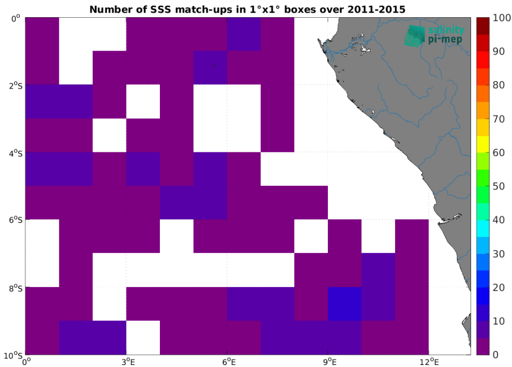
Figure 5: Number of SSS match-ups between Argo SSS and the Aquarius SSS L2 OR v5 (NASA-GSFC) SSS product for the Congo river plume Pi-MEP region over 1^\circ \times 1^\circ boxes and for the full satellite product period.
