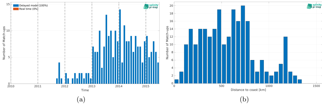
Figure 2: Number of match-ups between Argo and Aquarius SSS L2 OR v5 (NASA-GSFC) SSS as a function of time (a) and as function of the distance to coast (b) over the Congo river plume Pi-MEP region and for the full satellite product period.
