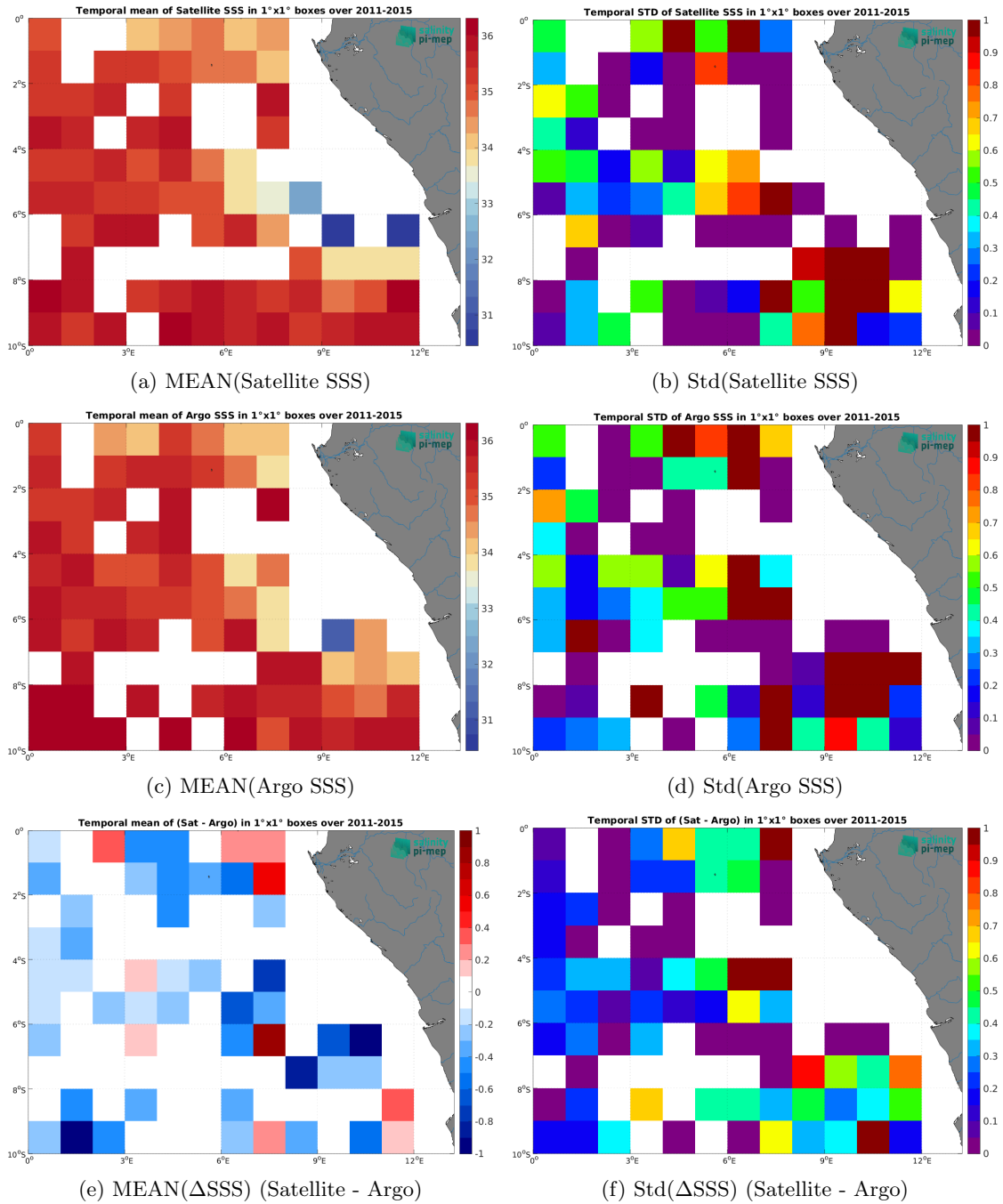
Figure 7: Temporal mean (left) and Std (right) of SSS from Aquarius SSS L2 OR v5 (NASA-GSFC) (top), Argo (middle), and of \Delta SSS (Satellite - Argo). Only match-up pairs are used to generate these maps.
