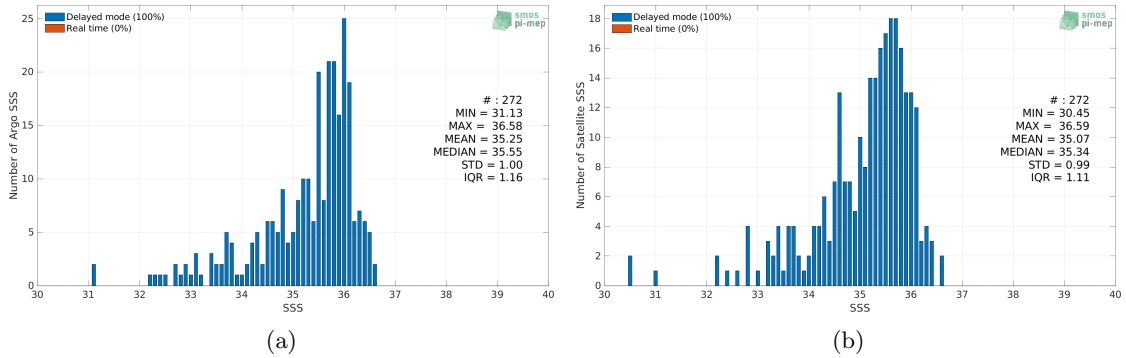
Figure 2: Histograms of SSS from Argo (a) and Aquarius SSS L2 OR v5 (NASA-GSFC) (b) considering all match-up pairs per bins of 0.1 over the Congo river plume Pi-MEP region and for the full satellite product period.
