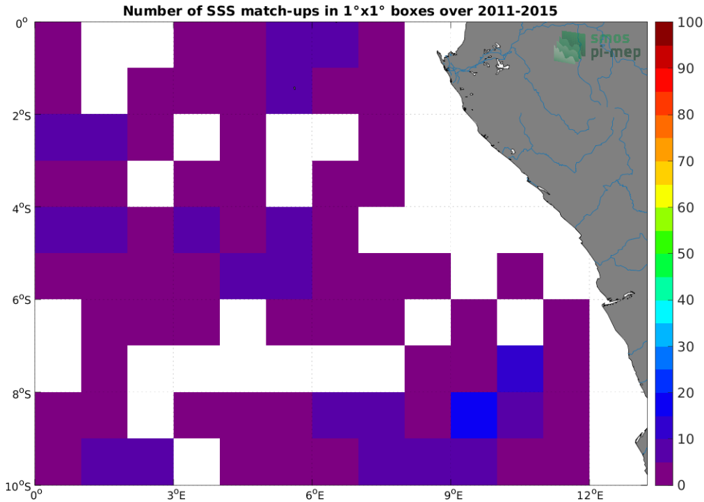
Figure 4: Number of SSS match-ups between Argo SSS and the Aquarius SSS L2 OR v5 (NASA-GSFC) SSS product for the Congo river plume Pi-MEP region over 1^\circ \times 1^\circ boxes and for the full satellite product period.
