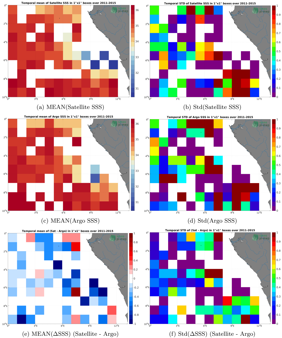
Figure 6: Temporal mean (left) and Std (right) of SSS from Aquarius SSS L2 OR v5 (NASA-GSFC) (top), Argo (middle), and of \Delta SSS (Satellite - Argo). Only match-up pairs are used to generate these maps.
