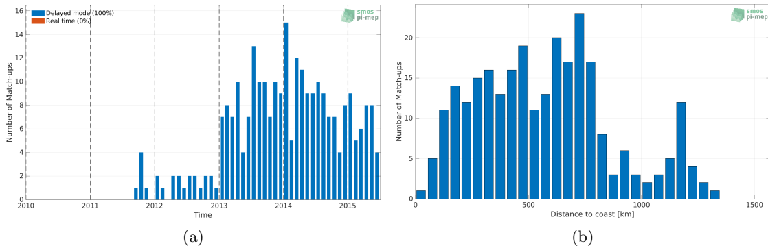
Figure 1: Number of match-ups between Argo and Aquarius SSS L2 OR v5 (NASA-GSFC) SSS as a function of time (a) and as function of the distance to coast (b) over the Congo river plume Pi-MEP region and for the full satellite product period.
