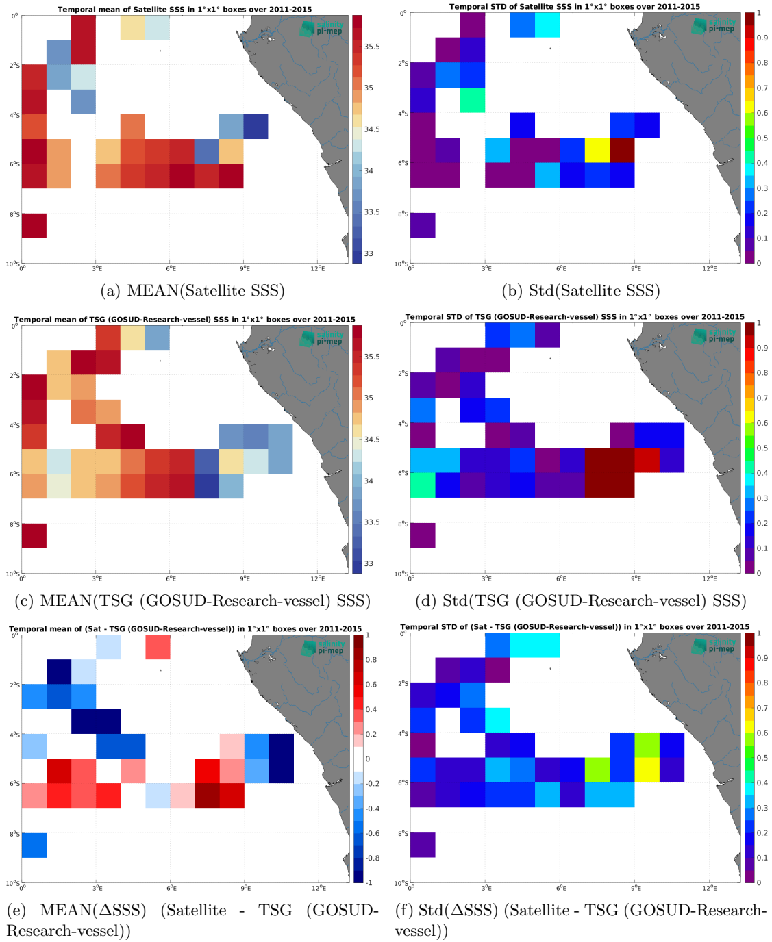
Figure 7: Temporal mean (left) and Std (right) of SSS from Aquarius SSS L2 CAP v5 (JPL) (top), TSG (GOSUD-Research-vessel) (middle), and of \Delta SSS (Satellite - TSG (GOSUD-Research-vessel)). Only match-up pairs are used to generate these maps.
