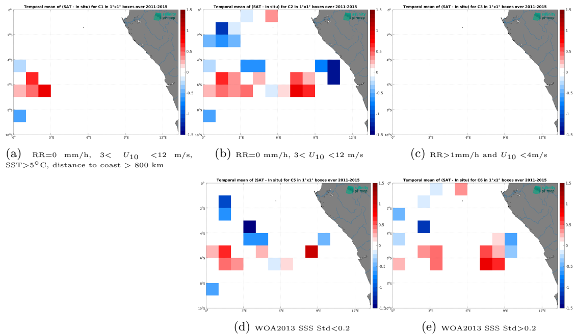
Figure 14: Temporal mean gridded over spatial boxes of size 1^\circ \times 1^\circ of \Delta SSS (Aquarius SSS L2 CAP v5 (JPL) - TSG (GOSUD-Research-vessel)) for 5 different subdatasets corresponding to:RR=0 mm/h, 3 < U_{10} < 12 m/s, SST>5°C, distance to coast > 800 km (a), RR=0 mm/h, 3 < U_{10} < 12 m/s (b), RR>1mm/h and U_{10} < 4 m/s (c), WOA2013 SSS Std<0.2 (d), WOA2013 SSS Std>0.2 (e).
