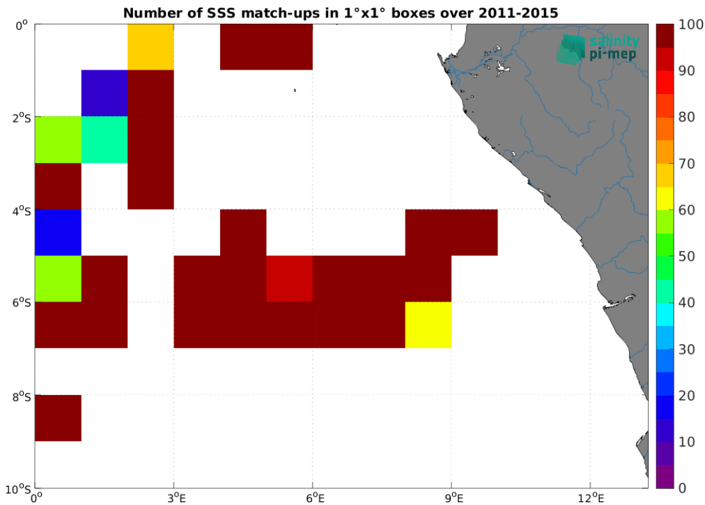
Figure 5: Number of SSS match-ups between TSG (GOSUD-Research-vessel) SSS and the Aquarius SSS L2 CAP v5 (JPL) SSS product for the Congo river plume Pi-MEP region over 1^\circ \times 1^\circ boxes and for the full satellite product period.
