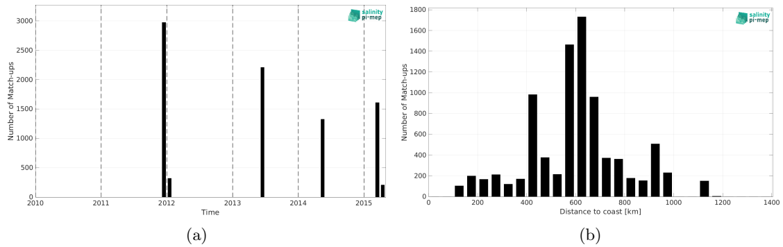
Figure 2: Number of match-ups between TSG (GOSUD-Research-vessel) and Aquarius SSS L2 CAP v5 (JPL) SSS as a function of time (a) and as function of the distance to coast (b) over the Congo river plume Pi-MEP region and for the full satellite product period.
