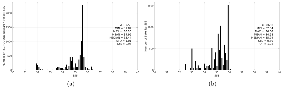
Figure 3: Histograms of SSS from TSG (GOSUD-Research-vessel) (a) and Aquarius SSS L2 CAP v5 (JPL) (b) considering all match-up pairs per bins of 0.1 over the Congo river plume Pi-MEP region and for the full satellite product period.
