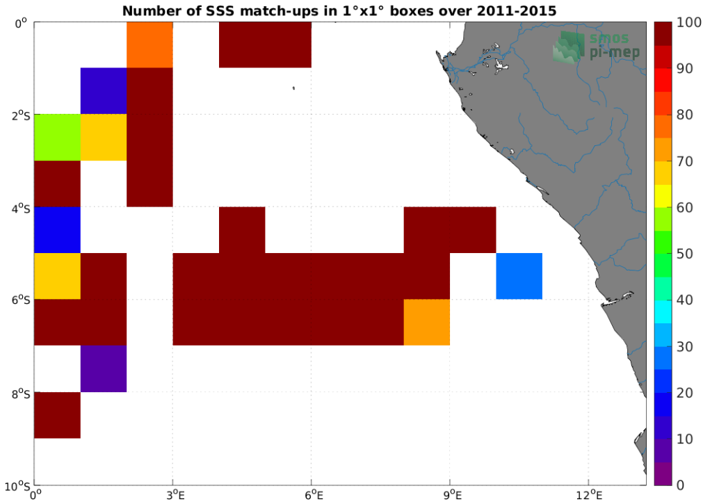
Figure 4: Number of SSS match-ups between TSG (GOSUD-Research-vessel) SSS and the Aquarius SSS L2 CAP v5 (JPL) SSS product for the Congo river plume Pi-MEP region over 1^\circ \times 1^\circ boxes and for the full satellite product period.
