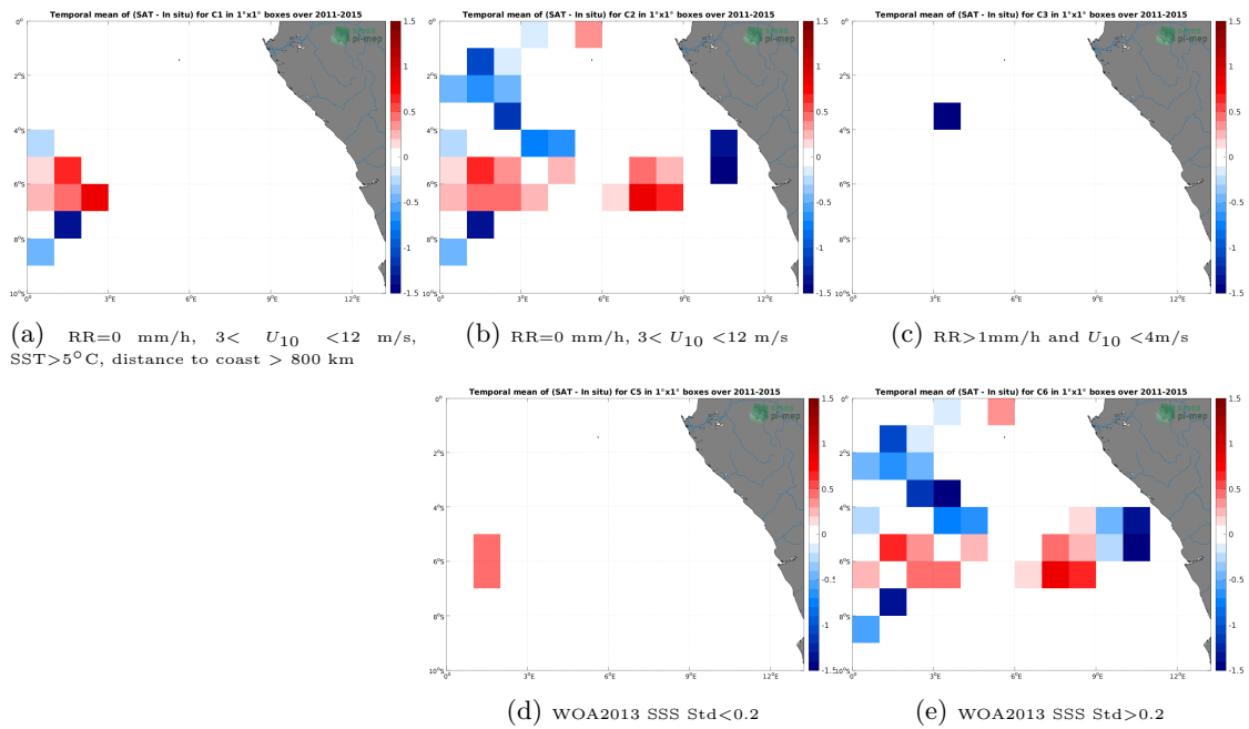
Figure 12: Temporal mean gridded over spatial boxes of size 1^\circ \times 1^\circ of \Delta SSS (Aquarius SSS L2 CAP v5 (JPL) - TSG (GOSUD-Research-vessel)) for 5 different subdatasets corresponding to:RR=0 mm/h, 3 < U_{10} < 12 m/s, SST>5°C, distance to coast > 800 km (a), RR=0 mm/h, 3 < U_{10} < 12 m/s (b), RR>1mm/h and U_{10} < 4 m/s (c), WOA2013 SSS Std<0.2 (d), WOA2013 SSS Std>0.2 (e).
