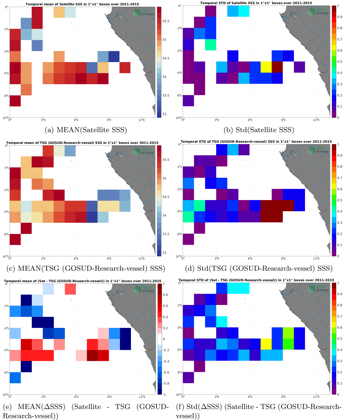
Figure 6: Temporal mean (left) and Std (right) of SSS from Aquarius SSS L2 CAP v5 (JPL) (top), TSG (GOSUD-Research-vessel) (middle), and of \Delta SSS (Satellite - TSG (GOSUD-Research-vessel)). Only match-up pairs are used to generate these maps.
