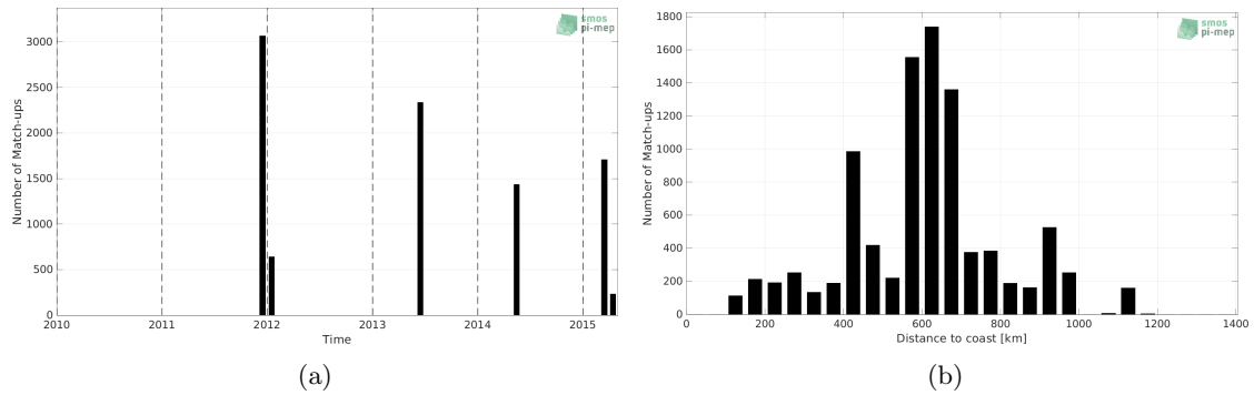
Figure 1: Number of match-ups between TSG (GOSUD-Research-vessel) and Aquarius SSS L2 CAP v5 (JPL) SSS as a function of time (a) and as function of the distance to coast (b) over the Congo river plume Pi-MEP region and for the full satellite product period.
