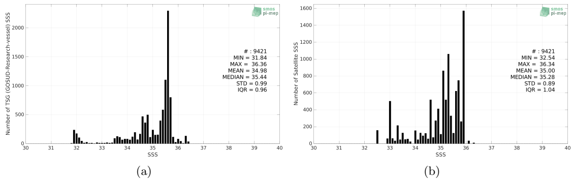
Figure 2: Histograms of SSS from TSG (GOSUD-Research-vessel) (a) and Aquarius SSS L2 CAP v5 (JPL) (b) considering all match-up pairs per bins of 0.1 over the Congo river plume Pi-MEP region and for the full satellite product period.
