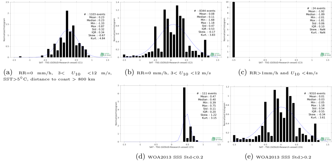
Figure 13: Normalized histogram of \Delta\text{SSS} (Aquarius SSS L2 CAP v5 (JPL) - TSG (GOSUD-Research-vessel)) for 5 different subdatasets corresponding to: RR=0 mm/h, 3 < U_{10} < 12 m/s, SST>5°C, distance to coast > 800 km (a), RR=0 mm/h, 3 < U_{10} < 12 m/s (b), RR>1mm/h and U_{10} < 4 m/s (c), WOA2013 SSS Std<0.2 (d), WOA2013 SSS Std>0.2 (e).
