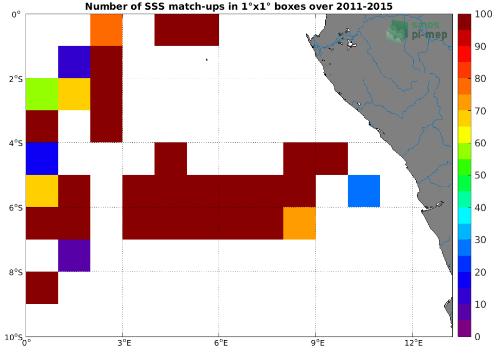
Figure 4: Number of SSS match-ups between TSG (GOSUD-Research-vessel) SSS and the Aquarius SSS L2 CAP v5 (JPL) SSS product for the Congo river plume Pi-MEP region over 1°x1° boxes and for the full satellite product period.
