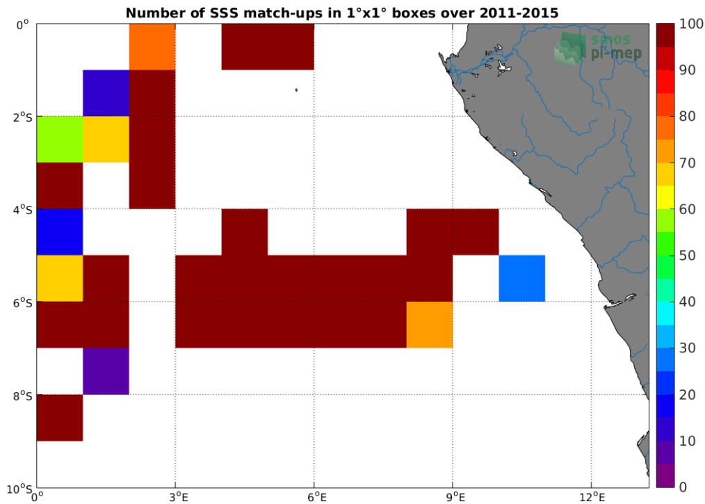
Figure 4: Number of SSS match-ups between TSG-GOSUD-Research-vessel SSS and the Aquarius-L2-JPL-V5 SSS product for the Congo river plume Pi-MEP region over 1^{\circ} \times 1^{\circ} boxes and for the full satellite product period.
