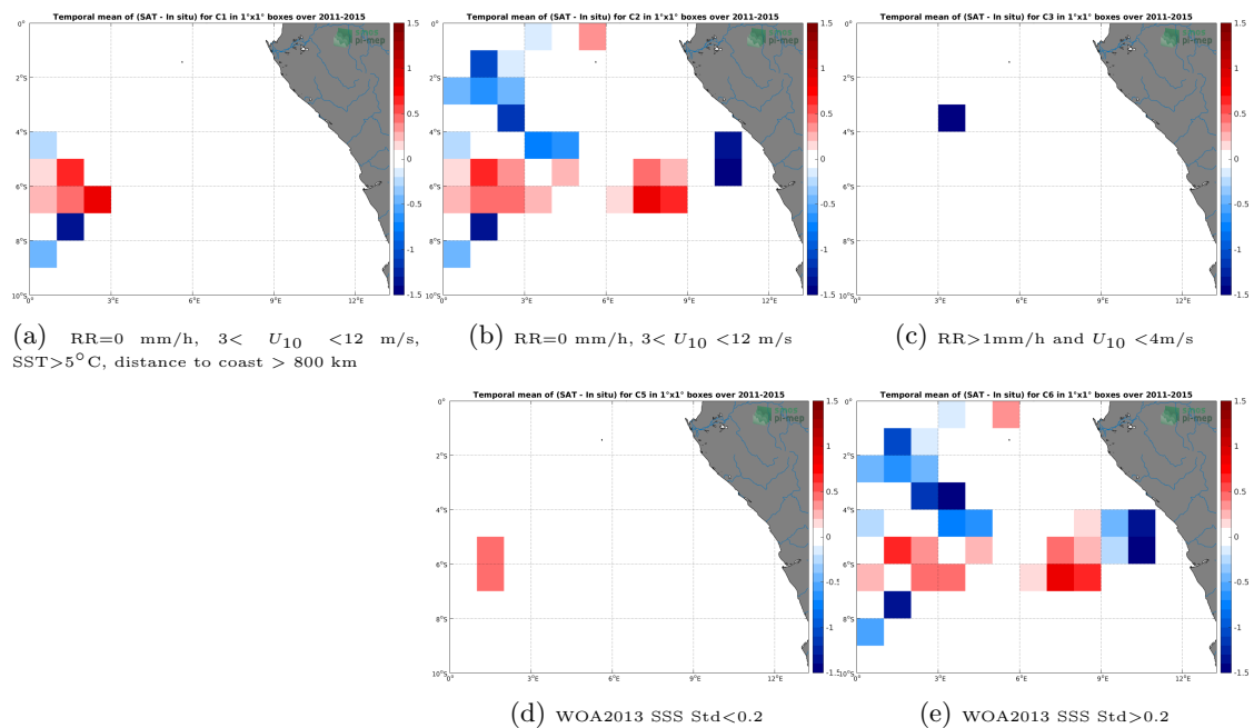
Figure 12: Temporal mean gridded over spatial boxes of size 1^\circ \times 1^\circ of \Delta SSS (Aquarius-L2-JPL-V5 - TSG-GOSUD-Research-vessel) for 5 different subdatasets corresponding to:RR=0 mm/h, 3 < U_{10} < 12 m/s, SST > 5^\circ\text{C} , distance to coast > 800 km (a), RR=0 mm/h, 3 < U_{10} < 12 m/s (b), RR > 1 mm/h and U_{10} < 4 m/s (c), WOA2013 SSS Std < 0.2 (d), WOA2013 SSS Std > 0.2 (e).
