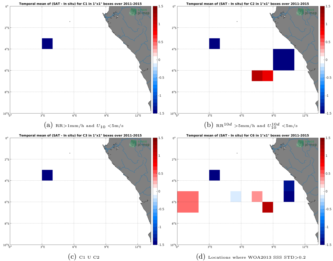
Figure 12: Temporal mean gridded over spatial boxes of size 1^\circ \times 1^\circ of \Delta SSS (Aquarius-L2-JPL-V5 - TSG-GOSUD-Research-vessel) for 4 different subdatasets corresponding to: RR > 1\text{mm/h} and U_{10} < 5\text{m/s} (a), RR^{10d} > 5\text{mm/h} and U_{10}^{10d} < 5\text{m/s} (b), C1 U C2 (c), Locations where WOA2013 SSS STD > 0.2 (d).
