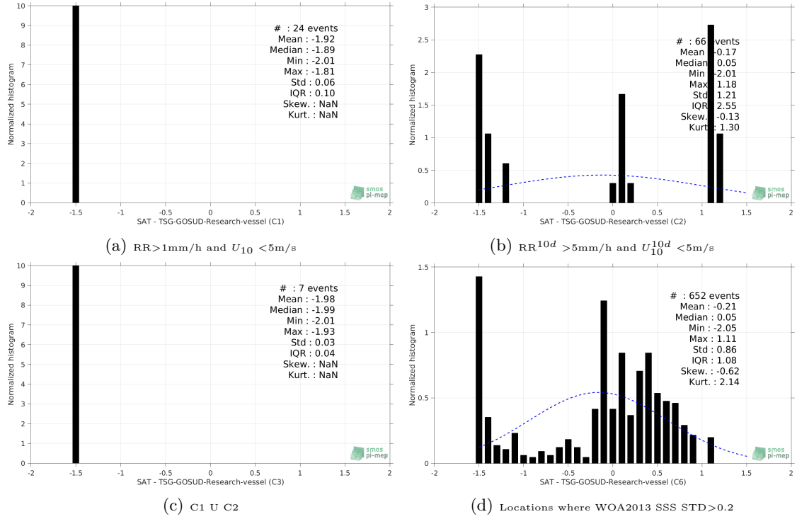
Figure 13: Normalized histogram of \Delta\text{SSS} (Aquarius-L2-JPL-V5 - TSG-GOSUD-Research-vessel) for 6 different subdatasets corresponding to: RR > 1mm/h and U_{10} < 5\text{m/s} (a), RR^{10d} > 5\text{mm/h} and U_{10}^{10d} < 5\text{m/s} (b), C1 U C2 (c), Locations where WOA2013 SSS STD > 0.2 (d).
