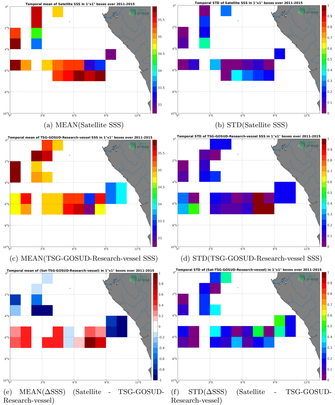
Figure 6: Temporal mean (left) and STD (right) of SSS from Aquarius-L2-JPL-V5 (top), TSG-GOSUD-Research-vessel (middle), and of \Delta SSS (Satellite - TSG-GOSUD-Research-vessel). Only match-up pairs are used to generate these maps.
