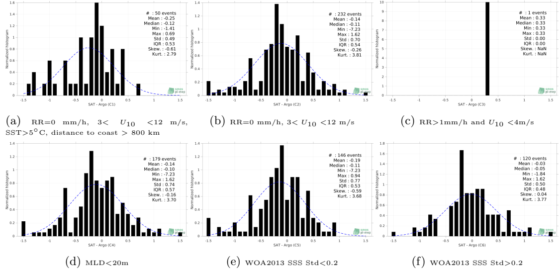
Figure 13: Normalized histogram of \Delta\text{SSS} (Aquarius SSS L2 CAP v5 (JPL) - Argo) for 6 different subdatasets corresponding to: RR=0 mm/h, 3 < U_{10} < 12 m/s, SST>5°C, distance to coast > 800 km (a), RR=0 mm/h, 3 < U_{10} < 12 m/s (b), RR>1mm/h and U_{10} < 4 m/s (c), MLD<20m (d), WOA2013 SSS Std<0.2 (e), WOA2013 SSS Std>0.2 (f).
