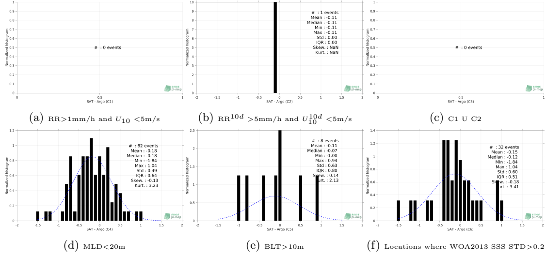
Figure 13: Normalized histogram of \Delta SSS (Aquarius-L2-JPL-V5 - Argo) for 6 different sub-datasets corresponding to: RR>1mm/h and U_{10} < 5\text{m/s} (a), RR^{10d} > 5\text{mm/h} and U_{10}^{10d} < 5\text{m/s} (b), C1 U C2 (c), MLD<20m (d), BLT>10m (e), Locations where WOA2013 SSS STD>0.2 (f).
