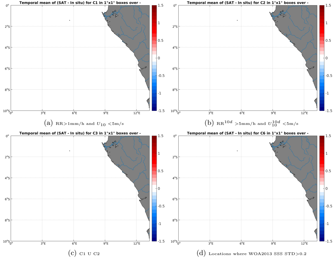
Figure 12: Temporal mean gridded over spatial boxes of size 1^\circ \times 1^\circ of \Delta SSS (AQUARIUS-L2-JPL-V4 - TSG-SAMOS) for 4 different subdatasets corresponding to: RR > 1 mm/h and U_{10} < 5 m/s (a), RR^{10d} > 5 mm/h and U_{10}^{10d} < 5 m/s (b), C1 U C2 (c), Locations where WOA2013 SSS STD > 0.2 (d).
