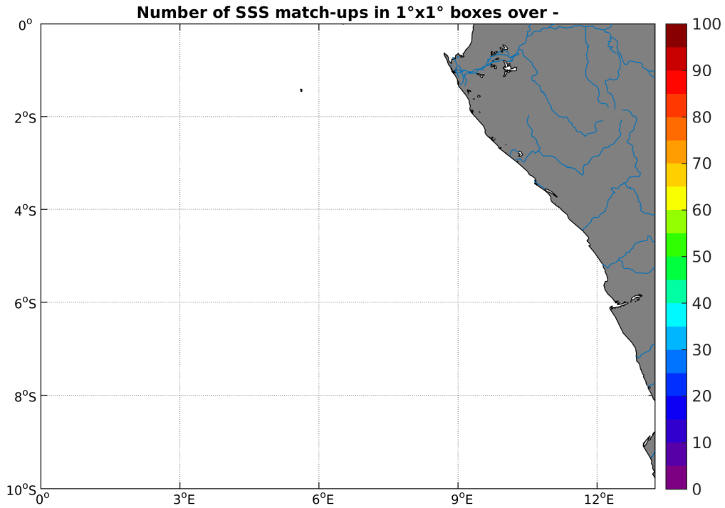
Figure 4: Number of SSS match-ups between TSG-SAMOS SSS and the AQUARIUS-L2-JPL-V4 SSS product for the Congo river plume Pi-MEP region over 1°x1° boxes and for the full satellite product period.
