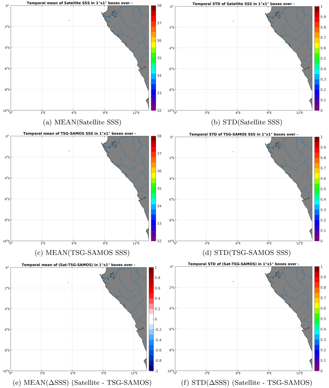
Figure 6: Temporal mean (left) and STD (right) of SSS from AQUARIUS-L2-JPL-V4 (top), TSG-SAMOS (middle), and of \Delta SSS (Satellite - TSG-SAMOS). Only match-up pairs are used to generate these maps.
