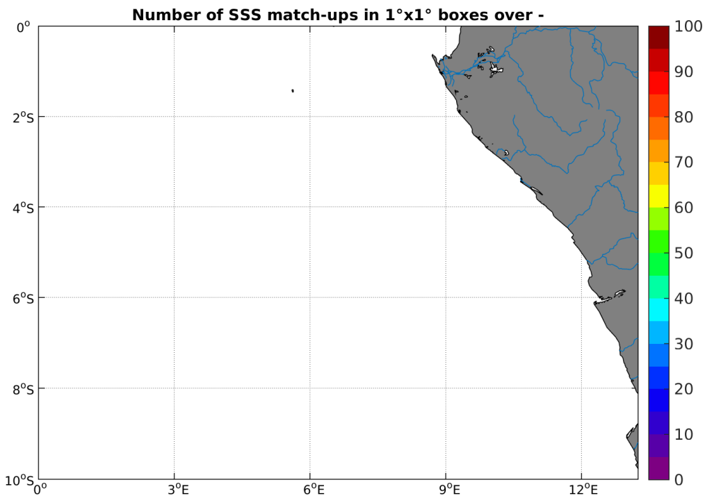
Figure 4: Number of SSS match-ups between TSG-GOSUD-Sailing-ship SSS and the AQUARIUS-L2-JPL-V4 SSS product for the Congo river plume Pi-MEP region over 1°x1° boxes and for the full satellite product period.
