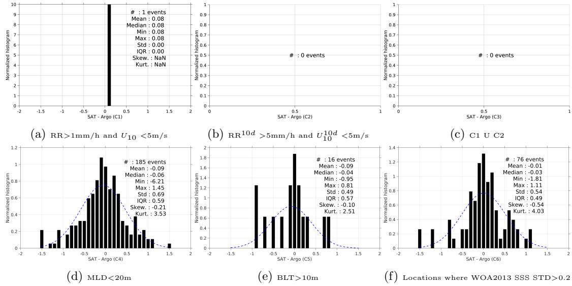
Figure 13: Normalized histogram of \Delta SSS (AQUARIUS-L2-JPL-V4 - Argo) for 6 different sub-datasets corresponding to: RR>1mm/h and U_{10} < 5\text{m/s} (a), RR 10d >5mm/h and U_{10}^{10d} < 5\text{m/s} (b), C1 U C2 (c),MLD<20m (d),BLT>10m (e),Locations where WOA2013 SSS STD>0.2 (f).
