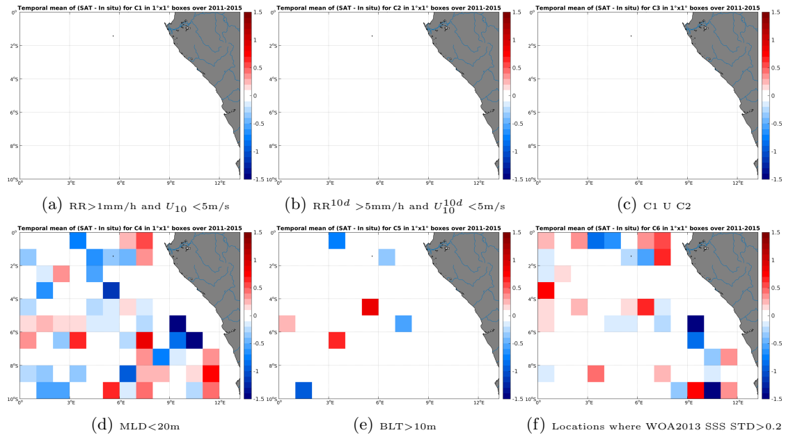
Figure 12: Temporal mean gridded over spatial boxes of size 1^\circ \times 1^\circ of \Delta SSS (AQUARIUS-L2-JPL-V4 - Argo) for 6 different subdatasets corresponding to: RR > 1\text{mm/h} and U_{10} < 5\text{m/s} (a), RR^{10d} > 5\text{mm/h} and U_{10}^{10d} < 5\text{m/s} (b), C1 U C2 (c), MLD < 20\text{m} (d), BLT > 10\text{m} (e), Locations where WOA2013 SSS STD > 0.2 (f).
