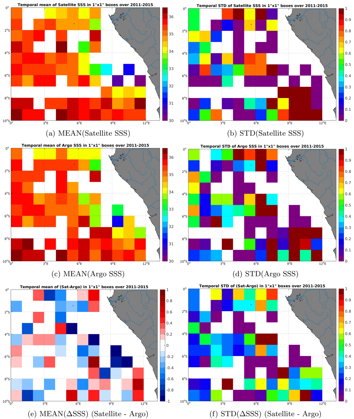
Figure 6: Temporal mean (left) and STD (right) of SSS from AQUARIUS-L2-JPL-V4 (top), Argo (middle), and of \Delta SSS (Satellite - Argo). Only match-up pairs are used to generate these maps.
