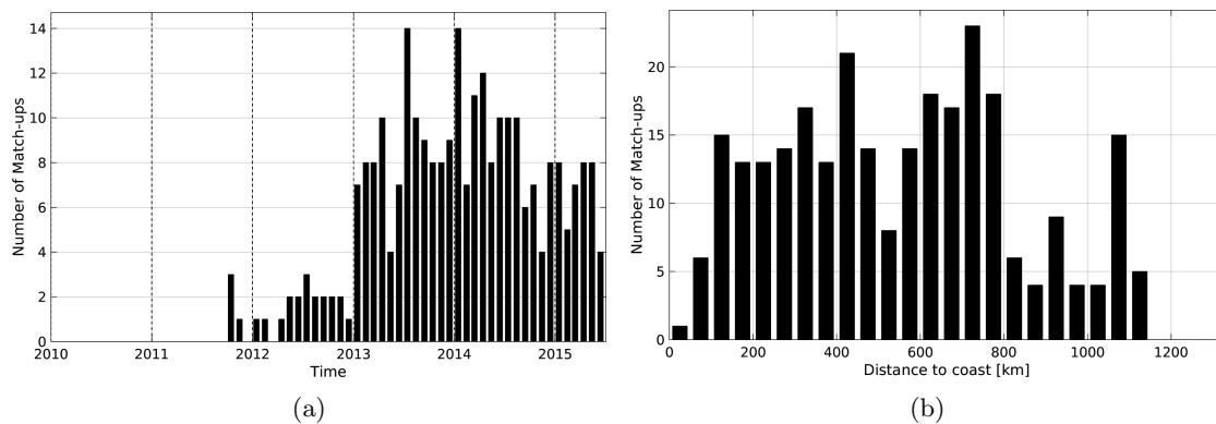
Figure 1: Number of match-ups between Argo and AQUARIUS-L2-JPL-V4 SSS as a function of time (a) and as function of the distance to coast (b) over the Congo river plume Pi-MEP region and for the full satellite product period.
