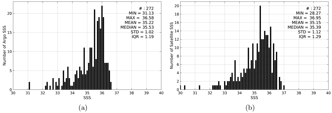
Figure 2: Histograms of SSS from Argo (a) and AQUARIUS-L2-JPL-V4 (b) considering all match-up pairs per bins of 0.1 over the Congo river plume Pi-MEP region and for the full satellite product period.
