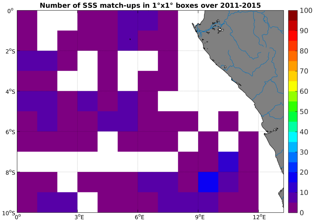
Figure 4: Number of SSS match-ups between Argo SSS and the AQUARIUS-L2-JPL-V4 SSS product for the Congo river plume Pi-MEP region over 1°x1° boxes and for the full satellite product period.
