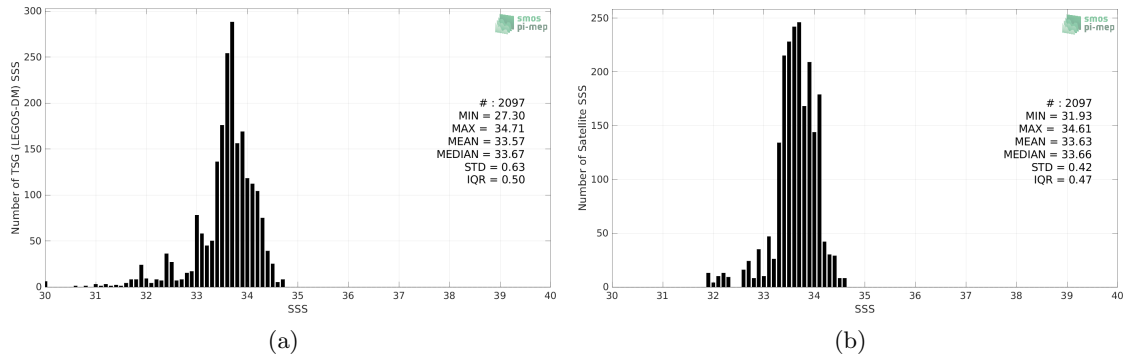
Figure 2: Histograms of SSS from TSG (LEGOS-DM) (a) and SMOS and SMAP SSS L4 OI v1 - 7 Days (LOPS) (b) considering all match-up pairs per bins of 0.1 over the Bay of Bengal Pi-MEP region and for the full satellite product period.
