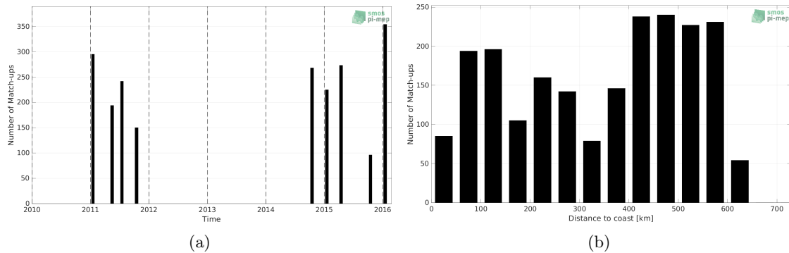
Figure 1: Number of match-ups between TSG (LEGOS-DM) and SMOS and SMAP SSS L4 OI v1 - 7 Days (LOPS) SSS as a function of time (a) and as function of the distance to coast (b) over the Bay of Bengal Pi-MEP region and for the full satellite product period.
