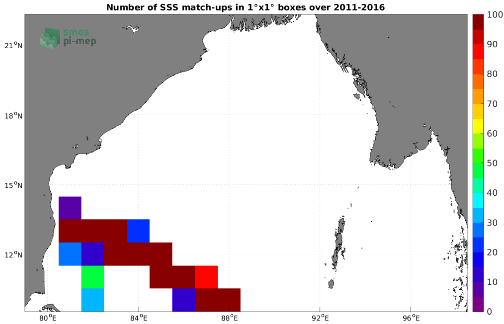
Figure 4: Number of SSS match-ups between TSG (LEGOS-DM) SSS and the SMOS and SMAP SSS L4 OI v1 - 7 Days (LOPS) SSS product for the Bay of Bengal Pi-MEP region over 1^\circ \times 1^\circ boxes and for the full satellite product period.
