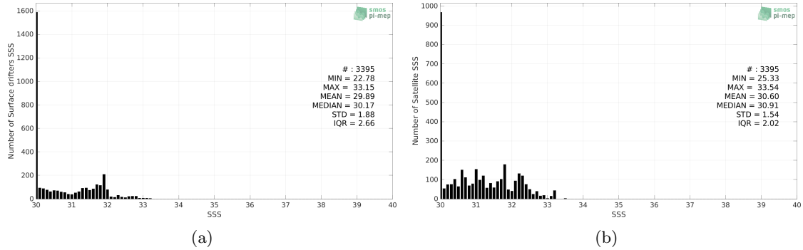
Figure 2: Histograms of SSS from Surface drifters (a) and SMOS and SMAP SSS L4 OI v1 - 7 Days (LOPS) (b) considering all match-up pairs per bins of 0.1 over the Bay of Bengal Pi-MEP region and for the full satellite product period.
