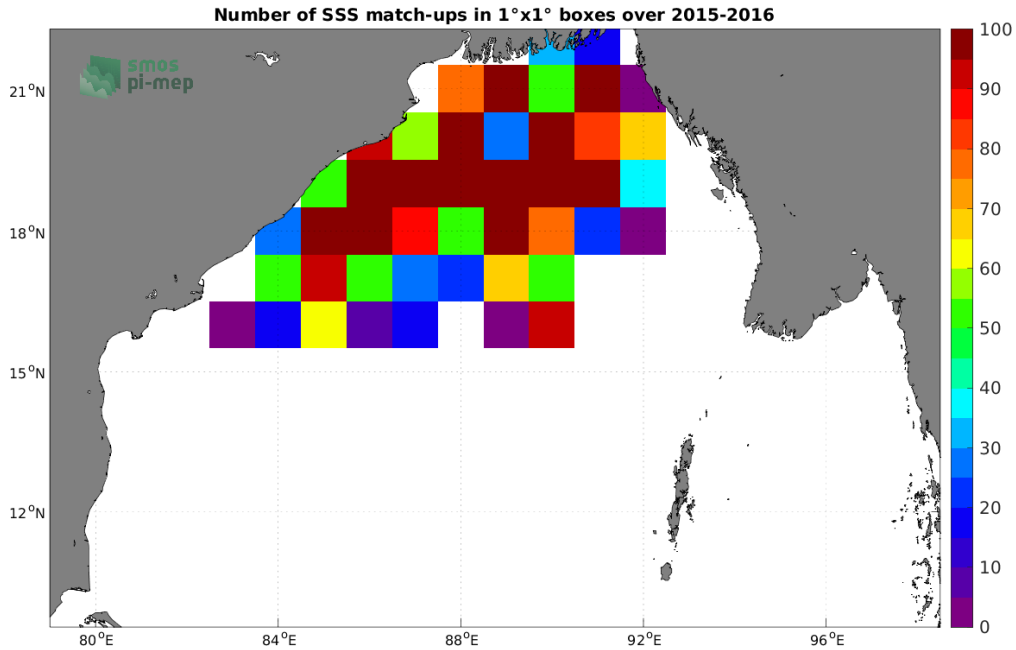
Figure 3: Number of SSS match-ups between Surface drifters SSS and the SMOS and SMAP SSS L4 OI v1 - 7 Days (LOPS) SSS product for the Bay of Bengal Pi-MEP region over 1^\circ \times 1^\circ boxes and for the full satellite product period.
