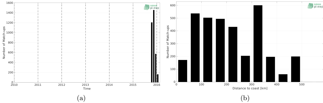
Figure 1: Number of match-ups between Surface drifters and SMOS and SMAP SSS L4 OI v1 - 7 Days (LOPS) SSS as a function of time (a) and as function of the distance to coast (b) over the Bay of Bengal Pi-MEP region and for the full satellite product period.
