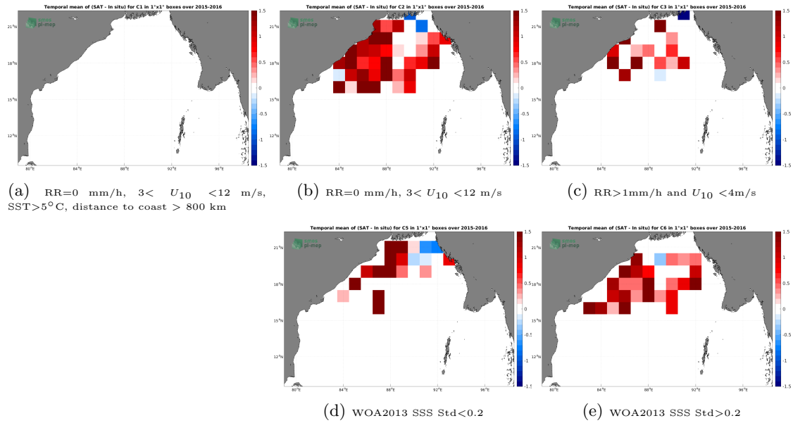
Figure 11: Temporal mean gridded over spatial boxes of size 1^\circ \times 1^\circ of \Delta\text{SSS} (SMOS and SMAP SSS L4 OI v1 - 7 Days (LOPS) - Surface drifters) for 5 different subdatasets corresponding to:RR=0 mm/h, 3 < U_{10} < 12 m/s, SST >5^\circ\text{C} , distance to coast > 800 km (a), RR=0 mm/h, 3 < U_{10} < 12 m/s (b), RR >1 mm/h and U_{10} < 4 m/s (c), WOA2013 SSS Std <0.2 (d), WOA2013 SSS Std >0.2 (e).
