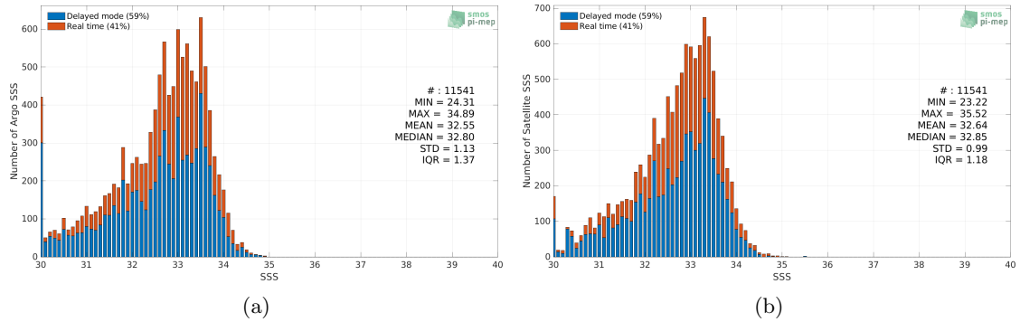
Figure 2: Histograms of SSS from Argo (a) and SMOS and SMAP SSS L4 OI v1 - 7 Days (LOPS) (b) considering all match-up pairs per bins of 0.1 over the Bay of Bengal Pi-MEP region and for the full satellite product period.
