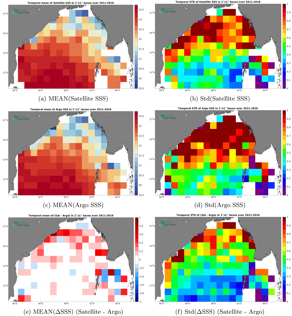
Figure 6: Temporal mean (left) and Std (right) of SSS from SMOS and SMAP SSS L4 OI v1 - 7 Days (LOPS) (top), Argo (middle), and of \Delta SSS (Satellite - Argo). Only match-up pairs are used to generate these maps.
