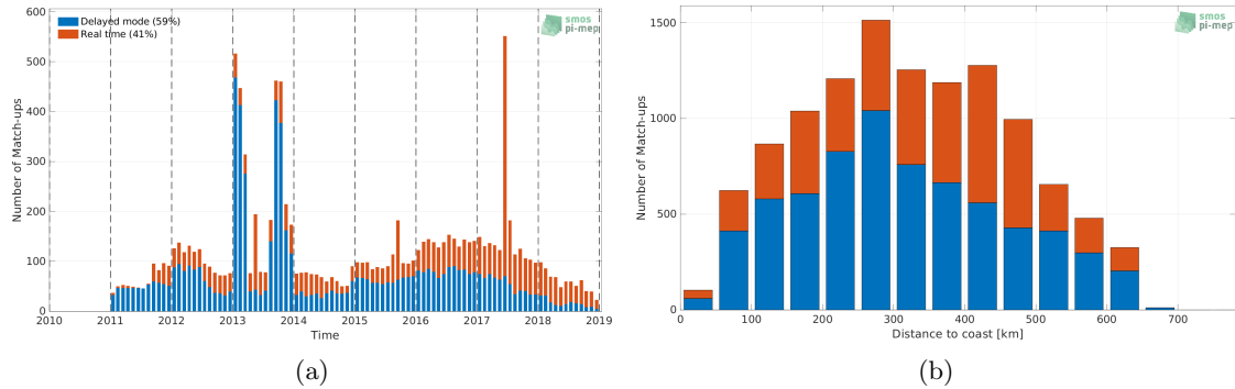
Figure 1: Number of match-ups between Argo and SMOS and SMAP SSS L4 OI v1 - 7 Days (LOPS) SSS as a function of time (a) and as function of the distance to coast (b) over the Bay of Bengal Pi-MEP region and for the full satellite product period.
