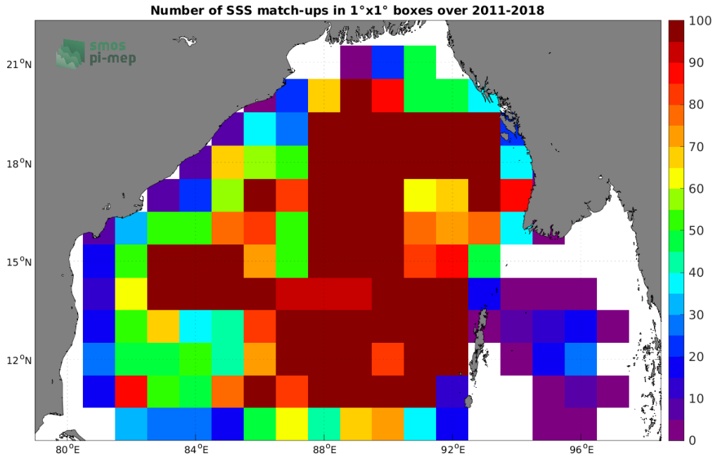
Figure 4: Number of SSS match-ups between Argo SSS and the SMOS and SMAP SSS L4 OI v1 - 7 Days (LOPS) SSS product for the Bay of Bengal Pi-MEP region over 1^\circ \times 1^\circ boxes and for the full satellite product period.
