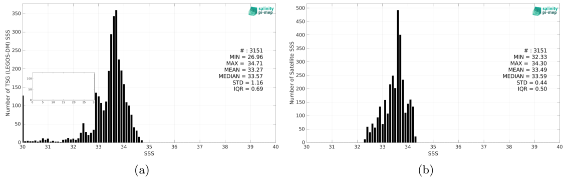
Figure 2: Histograms of SSS from TSG (LEGOS-DM) (a) and SMOS SSS L4 v1 - Weekly (CMEMS-CNR) (b) considering all match-up pairs per bins of 0.1 over the Bay of Bengal Pi-MEP region and for the full satellite product period.
