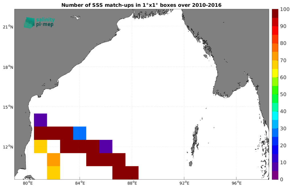
Figure 4: Number of SSS match-ups between TSG (LEGOS-DM) SSS and the SMOS SSS L4 v1 - Weekly (CMEMS-CNR) SSS product for the Bay of Bengal Pi-MEP region over 1^\circ \times 1^\circ boxes and for the full satellite product period.
