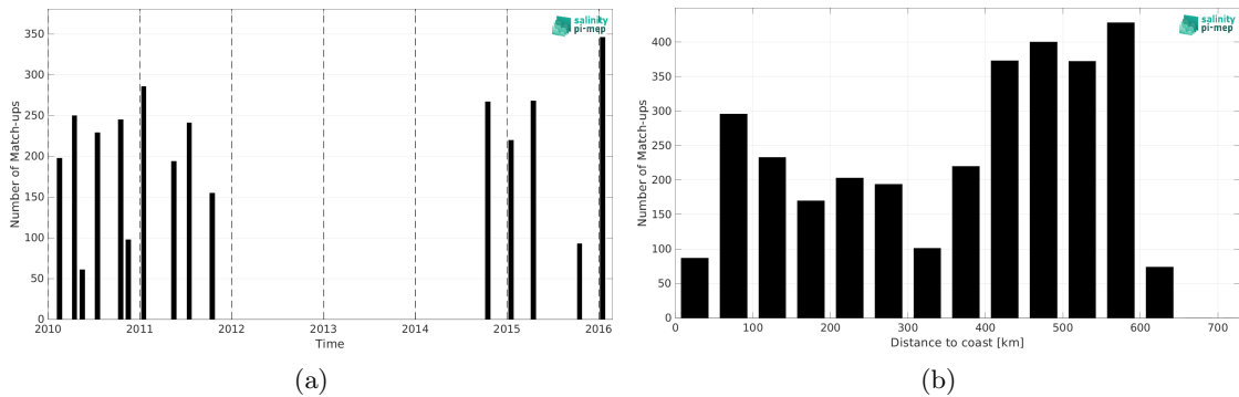
Figure 1: Number of match-ups between TSG (LEGOS-DM) and SMOS SSS L4 v1 - Weekly (CMEMS-CNR) SSS as a function of time (a) and as function of the distance to coast (b) over the Bay of Bengal Pi-MEP region and for the full satellite product period.
