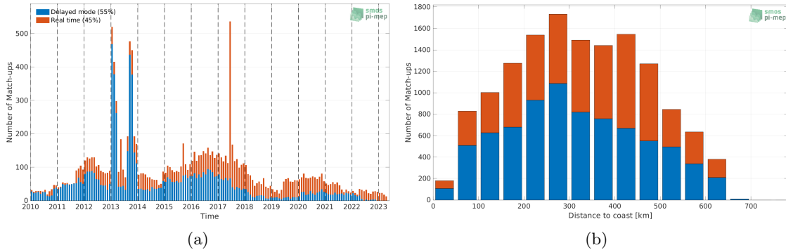
Figure 1: Number of match-ups between Argo and SMOS SSS L4 v1 - Weekly (CMEMS-CNR) SSS as a function of time (a) and as function of the distance to coast (b) over the Bay of Bengal Pi-MEP region and for the full satellite product period.
