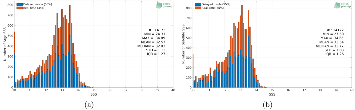
Figure 2: Histograms of SSS from Argo (a) and SMOS SSS L4 v1 - Weekly (CMEMS-CNR) (b) considering all match-up pairs per bins of 0.1 over the Bay of Bengal Pi-MEP region and for the full satellite product period.
