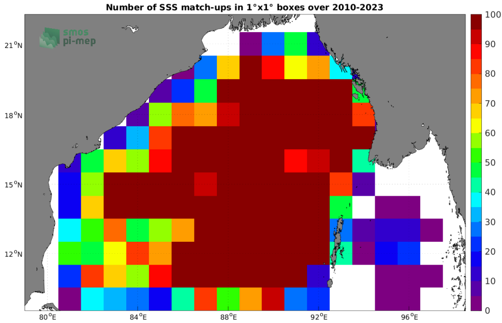
Figure 4: Number of SSS match-ups between Argo SSS and the SMOS SSS L4 v1 - Weekly (CMEMS-CNR) SSS product for the Bay of Bengal Pi-MEP region over 1^\circ \times 1^\circ boxes and for the full satellite product period.
