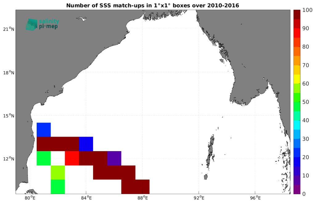
Figure 5: Number of SSS match-ups between TSG (LEGOS-DM) SSS and the SMOS SSS L4 v1 - Monthly (CMEMS-CNR) SSS product for the Bay of Bengal Pi-MEP region over 1^\circ \times 1^\circ boxes and for the full satellite product period.
