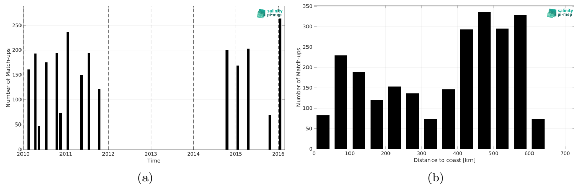
Figure 2: Number of match-ups between TSG (LEGOS-DM) and SMOS SSS L4 v1 - Monthly (CMEMS-CNR) SSS as a function of time (a) and as function of the distance to coast (b) over the Bay of Bengal Pi-MEP region and for the full satellite product period.
