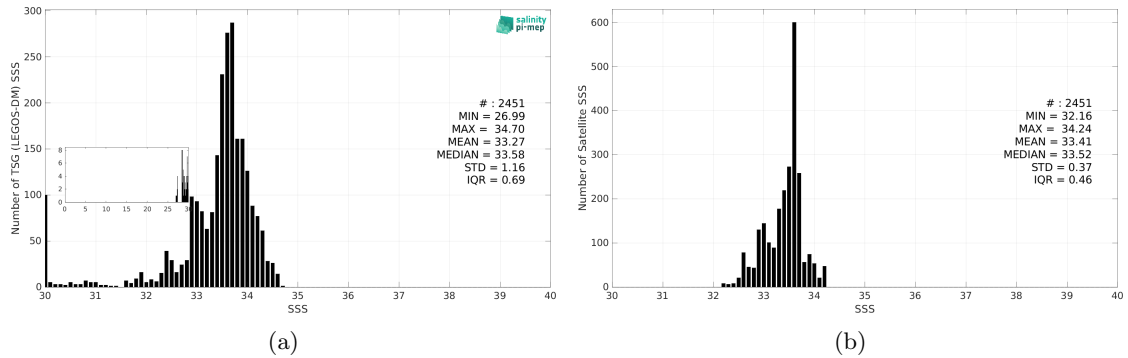
Figure 3: Histograms of SSS from TSG (LEGOS-DM) (a) and SMOS SSS L4 v1 - Monthly (CMEMS-CNR) (b) considering all match-up pairs per bins of 0.1 over the Bay of Bengal Pi-MEP region and for the full satellite product period.
