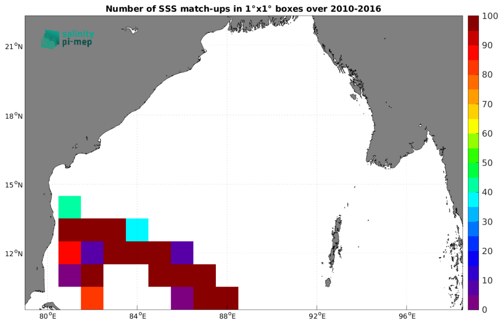
Figure 4: Number of SSS match-ups between TSG (LEGOS-DM) SSS and the SMOS SSS L4 v1 - Monthly (CMEMS-CNR) SSS product for the Bay of Bengal Pi-MEP region over 1^\circ \times 1^\circ boxes and for the full satellite product period.
