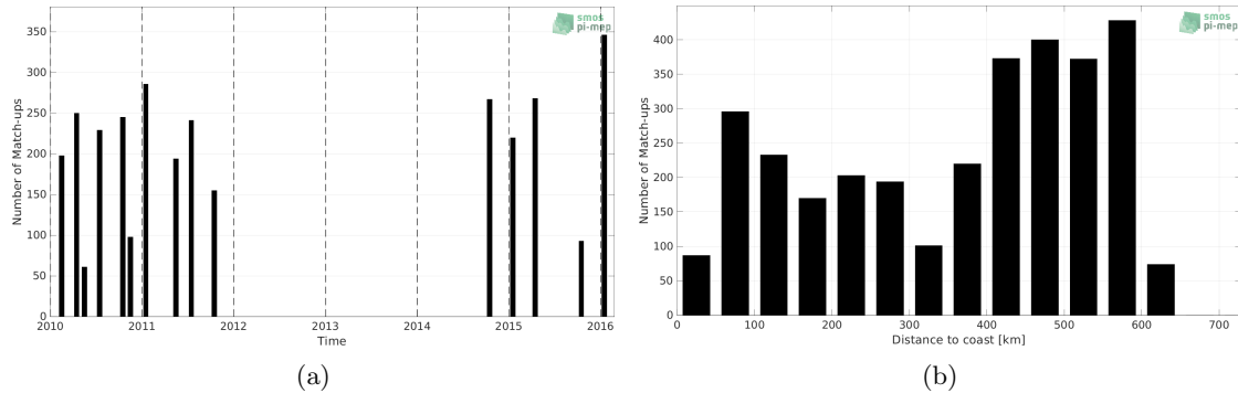
Figure 1: Number of match-ups between TSG (LEGOS-DM) and SMOS SSS L4 v1 - Monthly (CMEMS-CNR) SSS as a function of time (a) and as function of the distance to coast (b) over the Bay of Bengal Pi-MEP region and for the full satellite product period.
