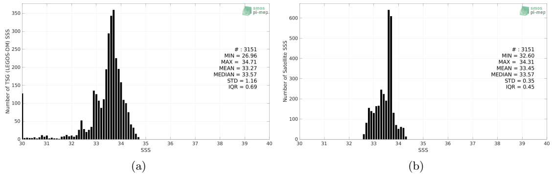
Figure 2: Histograms of SSS from TSG (LEGOS-DM) (a) and SMOS SSS L4 v1 - Monthly (CMEMS-CNR) (b) considering all match-up pairs per bins of 0.1 over the Bay of Bengal Pi-MEP region and for the full satellite product period.
