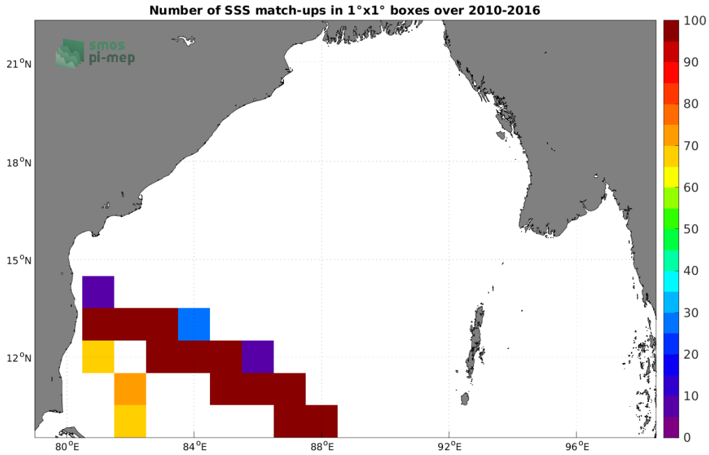
Figure 4: Number of SSS match-ups between TSG (LEGOS-DM) SSS and the SMOS SSS L4 v1 - Monthly (CMEMS-CNR) SSS product for the Bay of Bengal Pi-MEP region over 1°x1° boxes and for the full satellite product period.
