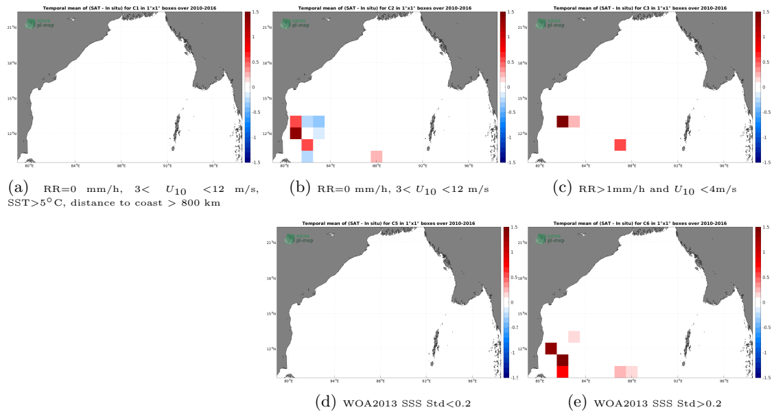
Figure 12: Temporal mean gridded over spatial boxes of size 1^\circ \times 1^\circ of \Delta SSS (SMOS SSS L4 v1 - Monthly (CMEMS-CNR) - TSG (LEGOS-DM)) for 5 different subdatasets corresponding to:RR=0 mm/h, 3 < U_{10} < 12 m/s, SST >5^\circ\text{C} , distance to coast > 800 km (a), RR=0 mm/h, 3 < U_{10} < 12 m/s (b), RR >1 mm/h and U_{10} < 4 m/s (c), WOA2013 SSS Std <0.2 (d), WOA2013 SSS Std >0.2 (e).
