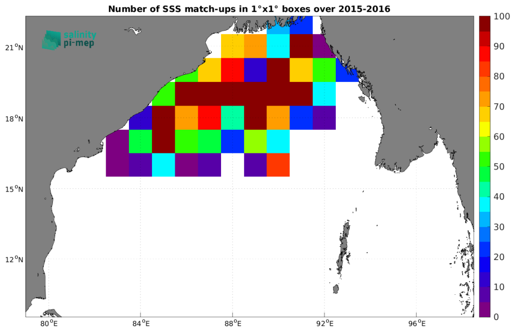
Figure 4: Number of SSS match-ups between Surface drifters SSS and the SMOS SSS L4 v1 - Monthly (CMEMS-CNR) SSS product for the Bay of Bengal Pi-MEP region over 1^\circ \times 1^\circ boxes and for the full satellite product period.
