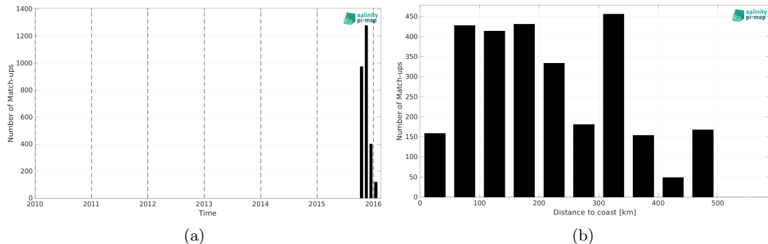
Figure 2: Number of match-ups between Surface drifters and SMOS SSS L4 v1 - Monthly (CMEMS-CNR) SSS as a function of time (a) and as function of the distance to coast (b) over the Bay of Bengal Pi-MEP region and for the full satellite product period.
