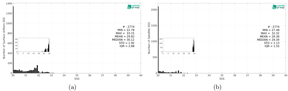
Figure 3: Histograms of SSS from Surface drifters (a) and SMOS SSS L4 v1 - Monthly (CMEMS-CNR) (b) considering all match-up pairs per bins of 0.1 over the Bay of Bengal Pi-MEP region and for the full satellite product period.
