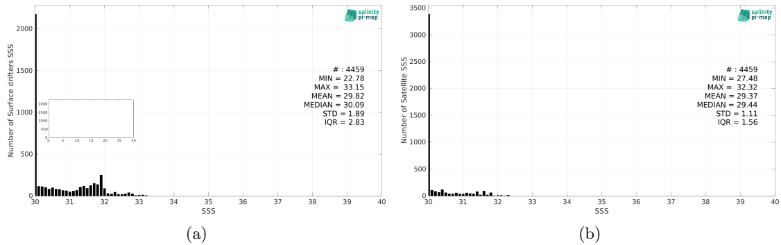
Figure 2: Histograms of SSS from Surface drifters (a) and SMOS SSS L4 v1 - Monthly (CMEMS-CNR) (b) considering all match-up pairs per bins of 0.1 over the Bay of Bengal Pi-MEP region and for the full satellite product period.
