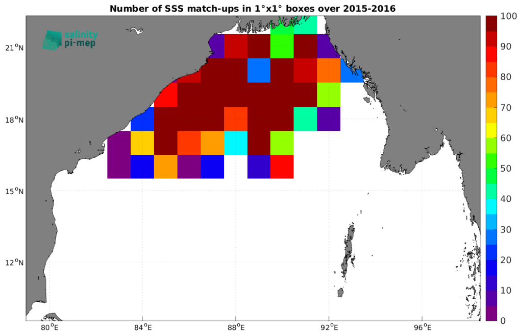
Figure 3: Number of SSS match-ups between Surface drifters SSS and the SMOS SSS L4 v1 - Monthly (CMEMS-CNR) SSS product for the Bay of Bengal Pi-MEP region over 1^\circ \times 1^\circ boxes and for the full satellite product period.
