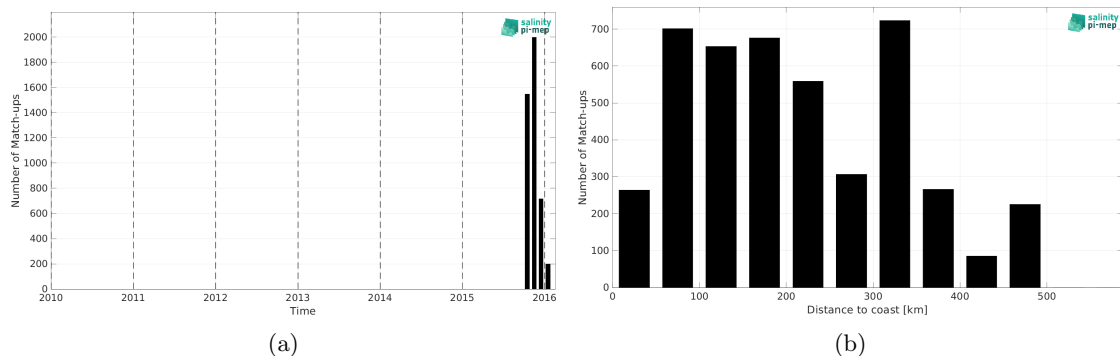
Figure 1: Number of match-ups between Surface drifters and SMOS SSS L4 v1 - Monthly (CMEMS-CNR) SSS as a function of time (a) and as function of the distance to coast (b) over the Bay of Bengal Pi-MEP region and for the full satellite product period.
