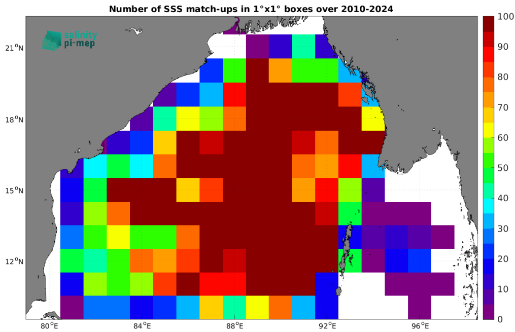
Figure 5: Number of SSS match-ups between Argo SSS and the SMOS SSS L4 v1 - Monthly (CMEMS-CNR) SSS product for the Bay of Bengal Pi-MEP region over 1^{\circ} \times 1^{\circ} boxes and for the full satellite product period.
