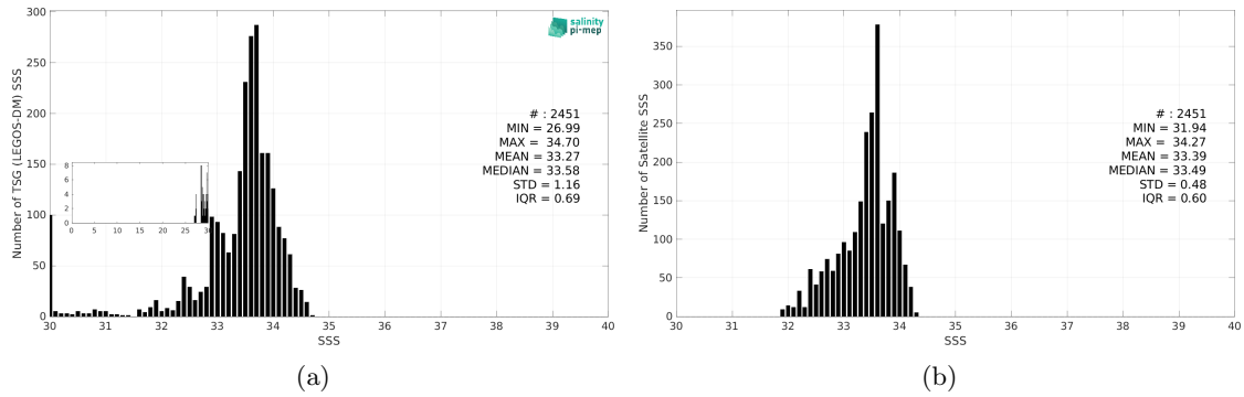
Figure 3: Histograms of SSS from TSG (LEGOS-DM) (a) and SMOS SSS L4 v1 - Daily (CMEMS-CNR) (b) considering all match-up pairs per bins of 0.1 over the Bay of Bengal Pi-MEP region and for the full satellite product period.
