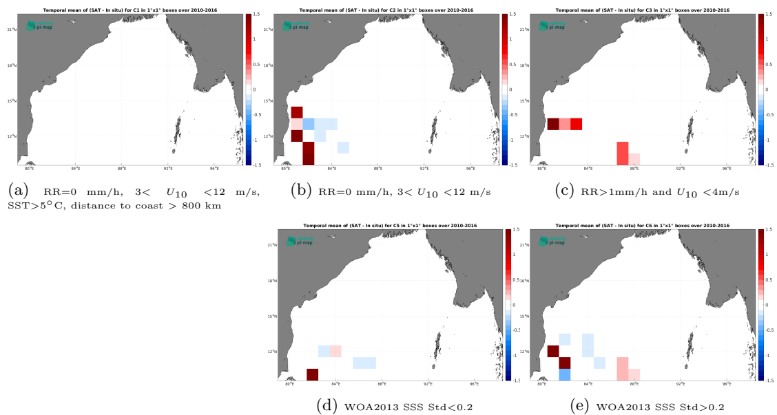
Figure 14: Temporal mean gridded over spatial boxes of size 1^\circ \times 1^\circ of \Delta\text{SSS} (SMOS SSS L4 v1 - Daily (CMEMS-CNR) - TSG (LEGOS-DM)) for 5 different subdatasets corresponding to:RR=0 mm/h, 3 < U_{10} < 12 m/s, SST >5^\circ\text{C} , distance to coast > 800 km (a), RR=0 mm/h, 3 < U_{10} < 12 m/s (b), RR >1 mm/h and U_{10} < 4 m/s (c), WOA2013 SSS Std <0.2 (d), WOA2013 SSS Std >0.2 (e).
