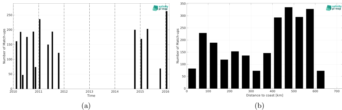
Figure 2: Number of match-ups between TSG (LEGOS-DM) and SMOS SSS L4 v1 - Daily (CMEMS-CNR) SSS as a function of time (a) and as function of the distance to coast (b) over the Bay of Bengal Pi-MEP region and for the full satellite product period.
