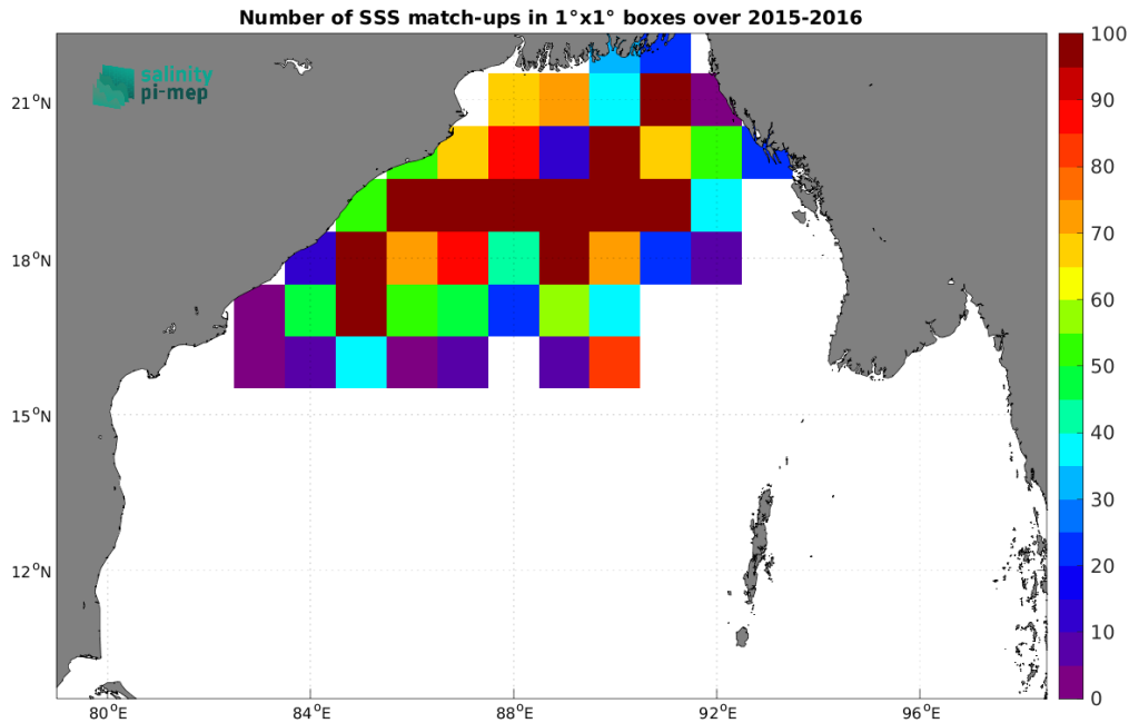
Figure 4: Number of SSS match-ups between Surface drifters SSS and the SMOS SSS L4 v1 - Daily (CMEMS-CNR) SSS product for the Bay of Bengal Pi-MEP region over 1^\circ \times 1^\circ boxes and for the full satellite product period.
