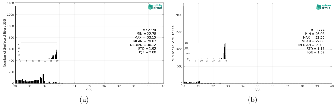
Figure 3: Histograms of SSS from Surface drifters (a) and SMOS SSS L4 v1 - Daily (CMEMS-CNR) (b) considering all match-up pairs per bins of 0.1 over the Bay of Bengal Pi-MEP region and for the full satellite product period.
