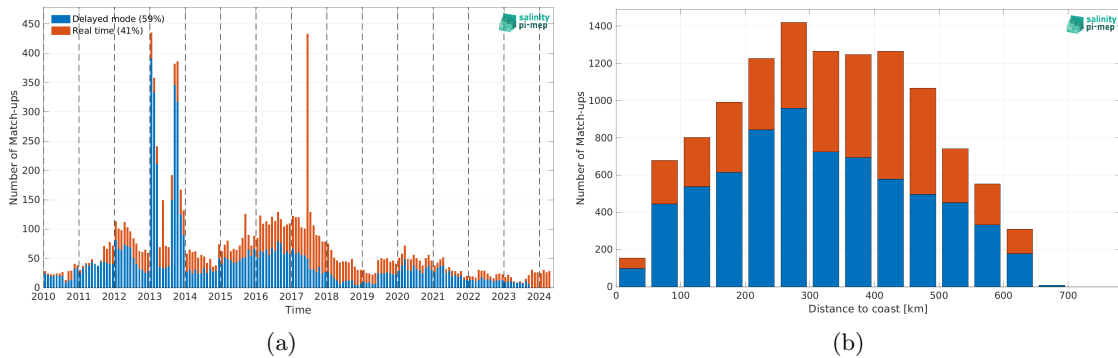
Figure 2: Number of match-ups between Argo and SMOS SSS L4 v1 - Daily (CMEMS-CNR) SSS as a function of time (a) and as function of the distance to coast (b) over the Bay of Bengal Pi-MEP region and for the full satellite product period.
