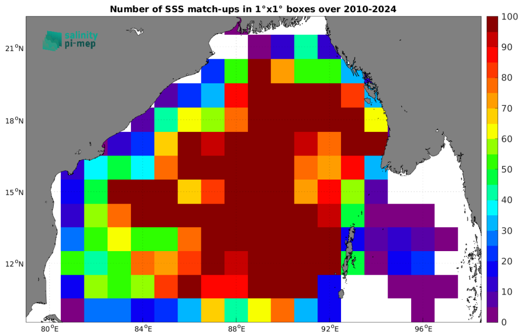
Figure 5: Number of SSS match-ups between Argo SSS and the SMOS SSS L4 v1 - Daily (CMEMS-CNR) SSS product for the Bay of Bengal Pi-MEP region over 1^{\circ} \times 1^{\circ} boxes and for the full satellite product period.
