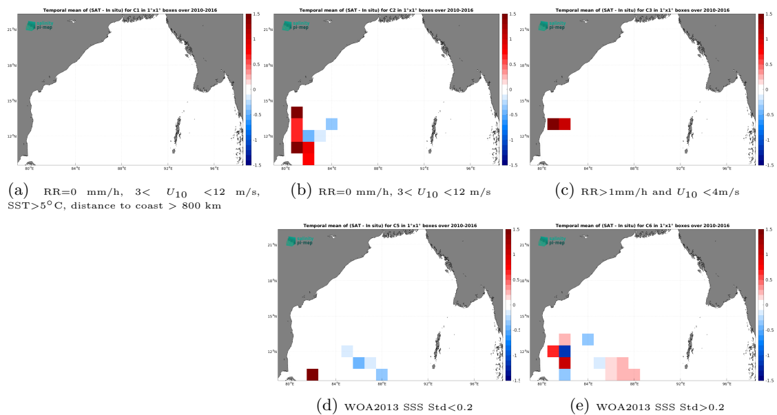
Figure 14: Temporal mean gridded over spatial boxes of size 1^\circ \times 1^\circ of \Delta\text{SSS} (SMOS SSS L4 OI v346 - Weekly (CMEMS-CATDS-LOPS) - TSG (LEGOS-DM)) for 5 different subdatasets corresponding to:RR=0 mm/h, 3 < U_{10} < 12 m/s, SST >5^\circ\text{C} , distance to coast > 800 km (a), RR=0 mm/h, 3 < U_{10} < 12 m/s (b), RR >1 mm/h and U_{10} < 4 m/s (c), WOA2013 SSS Std <0.2 (d), WOA2013 SSS Std >0.2 (e).
