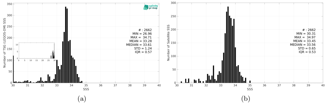
Figure 3: Histograms of SSS from TSG (LEGOS-DM) (a) and SMOS SSS L4 OI v346 - Weekly (CMEMS-CATDS-LOPS) (b) considering all match-up pairs per bins of 0.1 over the Bay of Bengal Pi-MEP region and for the full satellite product period.
