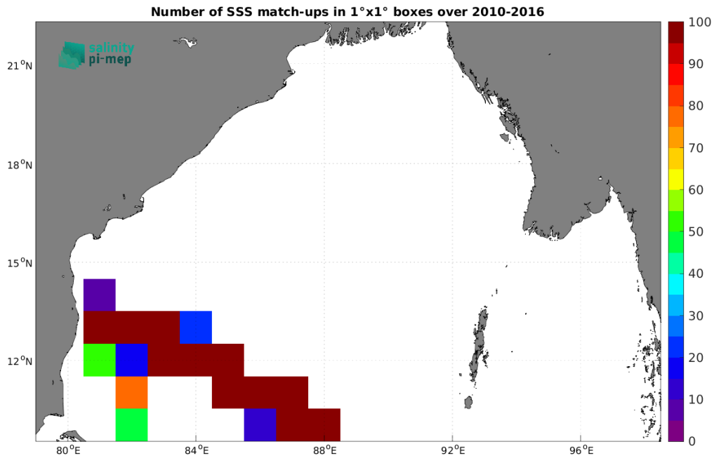
Figure 5: Number of SSS match-ups between TSG (LEGOS-DM) SSS and the SMOS SSS L4 OI v346 - Weekly (CMEMS-CATDS-LOPS) SSS product for the Bay of Bengal Pi-MEP region over 1^\circ \times 1^\circ boxes and for the full satellite product period.
