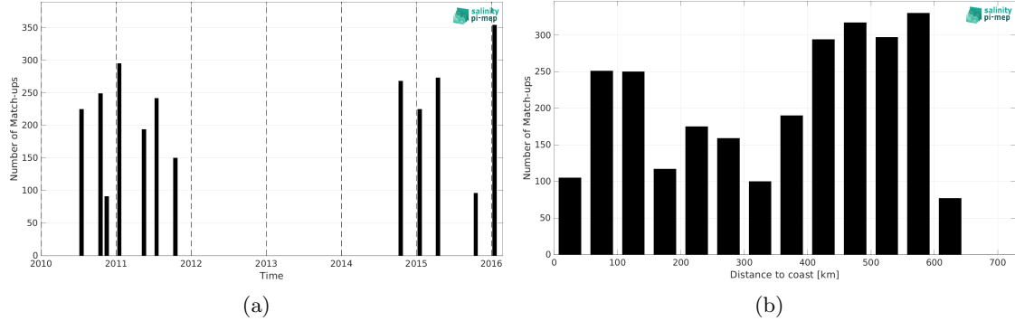
Figure 2: Number of match-ups between TSG (LEGOS-DM) and SMOS SSS L4 OI v346 - Weekly (CMEMS-CATDS-LOPS) SSS as a function of time (a) and as function of the distance to coast (b) over the Bay of Bengal Pi-MEP region and for the full satellite product period.
