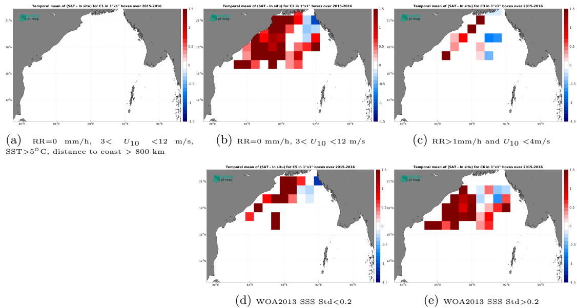
Figure 13: Temporal mean gridded over spatial boxes of size 1^\circ \times 1^\circ of \Delta\text{SSS} (SMOS SSS L4 OI v346 - Weekly (CMEMS-CATDS-LOPS) - Surface drifters) for 5 different subdatasets corresponding to:RR=0 mm/h, 3 < U_{10} < 12 m/s, SST >5^\circ\text{C} , distance to coast > 800 km (a), RR=0 mm/h, 3 < U_{10} < 12 m/s (b), RR >1 mm/h and U_{10} < 4 m/s (c), WOA2013 SSS Std <0.2 (d), WOA2013 SSS Std >0.2 (e).
