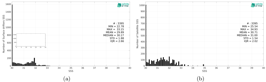
Figure 2: Histograms of SSS from Surface drifters (a) and SMOS SSS L4 OI v342 - Weekly (CMEMS-CATDS-LOPS) (b) considering all match-up pairs per bins of 0.1 over the Bay of Bengal Pi-MEP region and for the full satellite product period.
