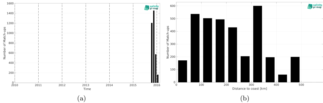
Figure 1: Number of match-ups between Surface drifters and SMOS SSS L4 OI v342 - Weekly (CMEMS-CATDS-LOPS) SSS as a function of time (a) and as function of the distance to coast (b) over the Bay of Bengal Pi-MEP region and for the full satellite product period.
