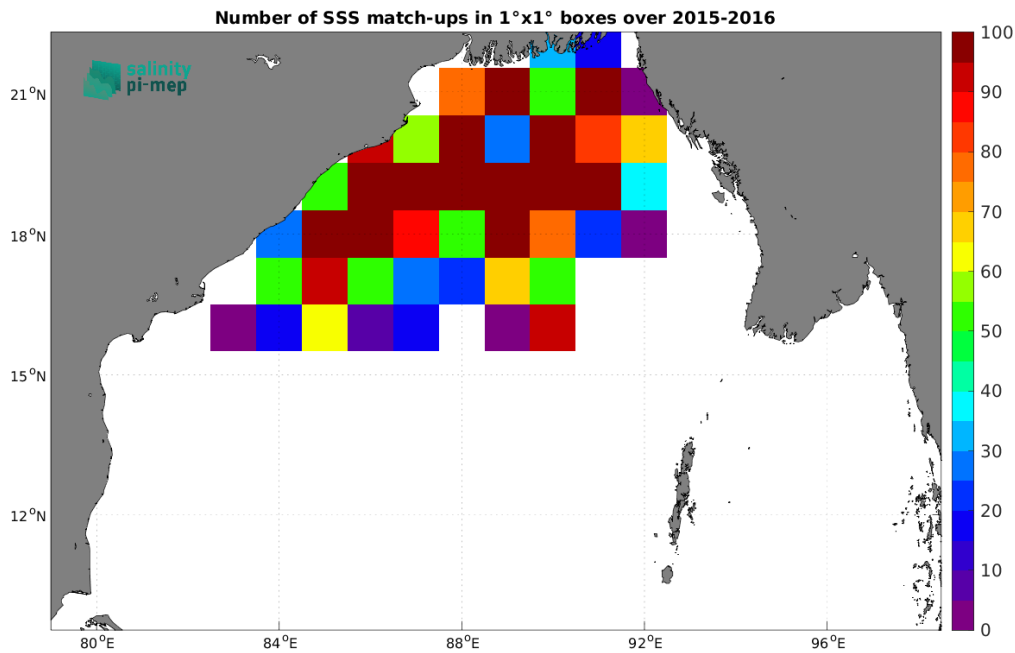
Figure 3: Number of SSS match-ups between Surface drifters SSS and the SMOS SSS L4 OI v342 - Weekly (CMEMS-CATDS-LOPS) SSS product for the Bay of Bengal Pi-MEP region over 1^\circ \times 1^\circ boxes and for the full satellite product period.
