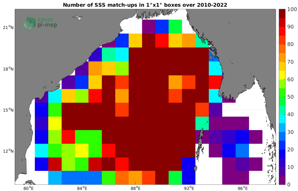
Figure 4: Number of SSS match-ups between Argo SSS and the SMOS SSS L4 OI v342 - Weekly (CMEMS-CATDS-LOPS) SSS product for the Bay of Bengal Pi-MEP region over 1°x1° boxes and for the full satellite product period.
